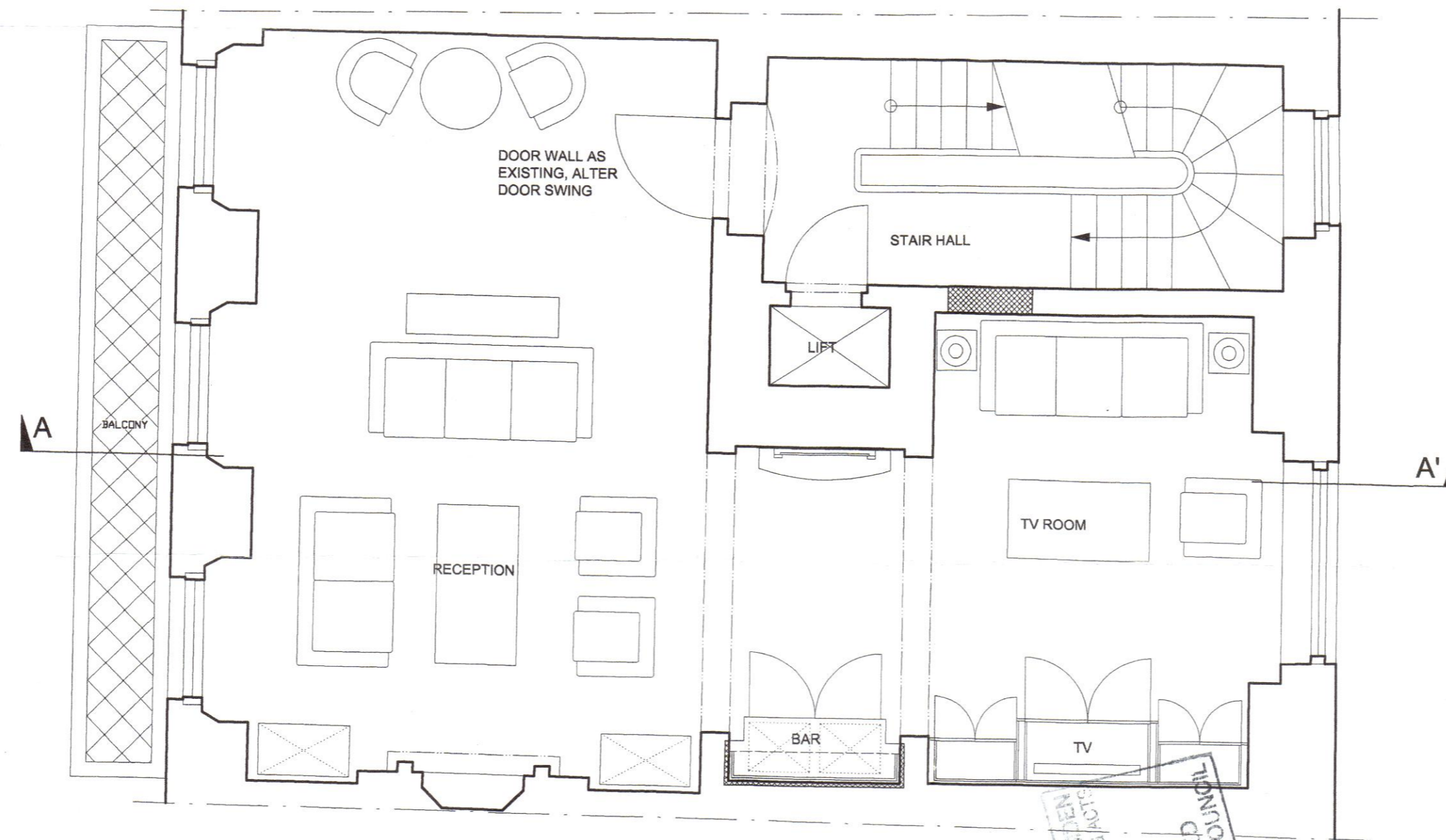
PROPOSED / CONSTRUCTION PLAN: FIRST FLOOR
