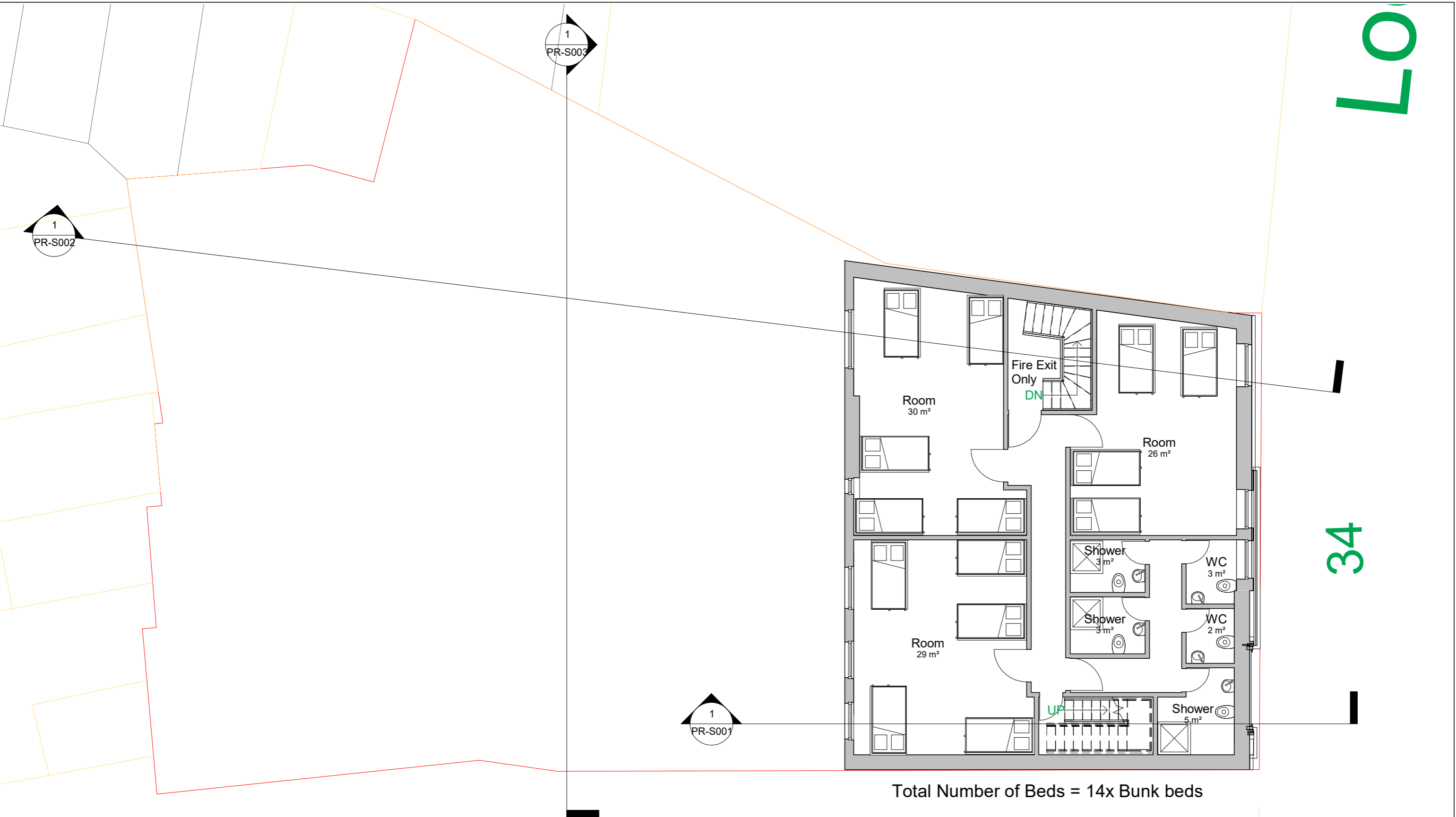
1 Third Floor Plan 1 : 100
