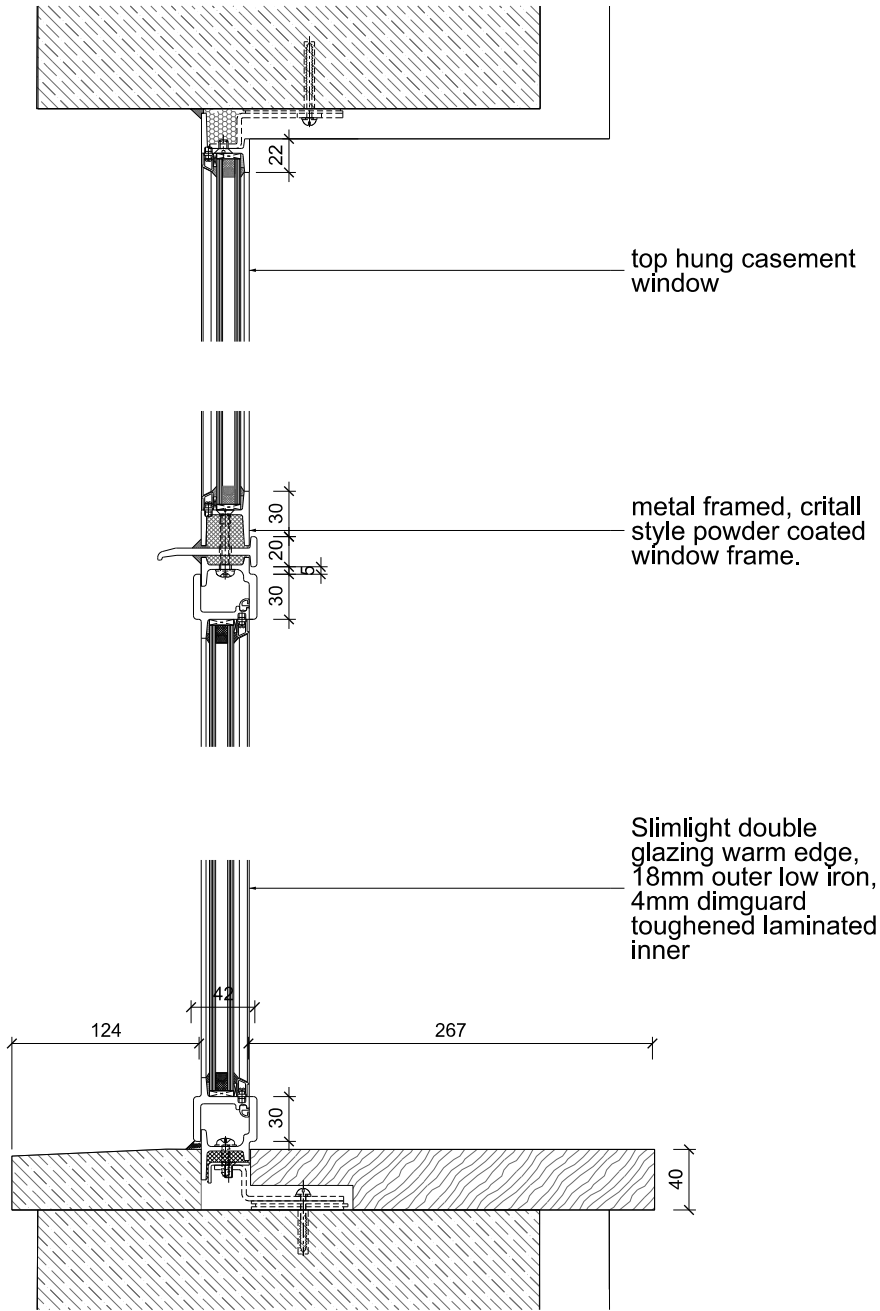
02 (00)300 No 19 Denmark Street Window Section detail 1:5
