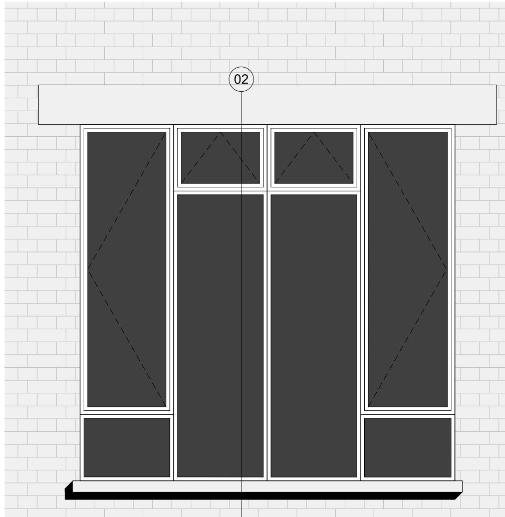
01 (00)300 No 19 Denmark Street Window Elevation 1:20
