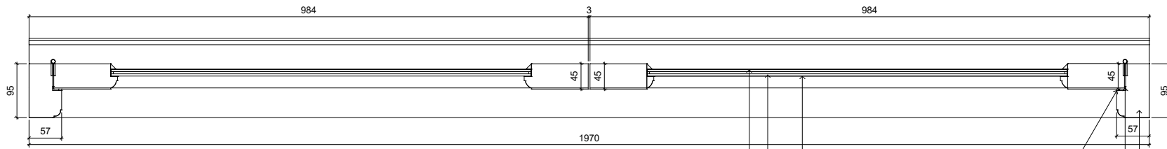
3 Detail Plan 1:3
