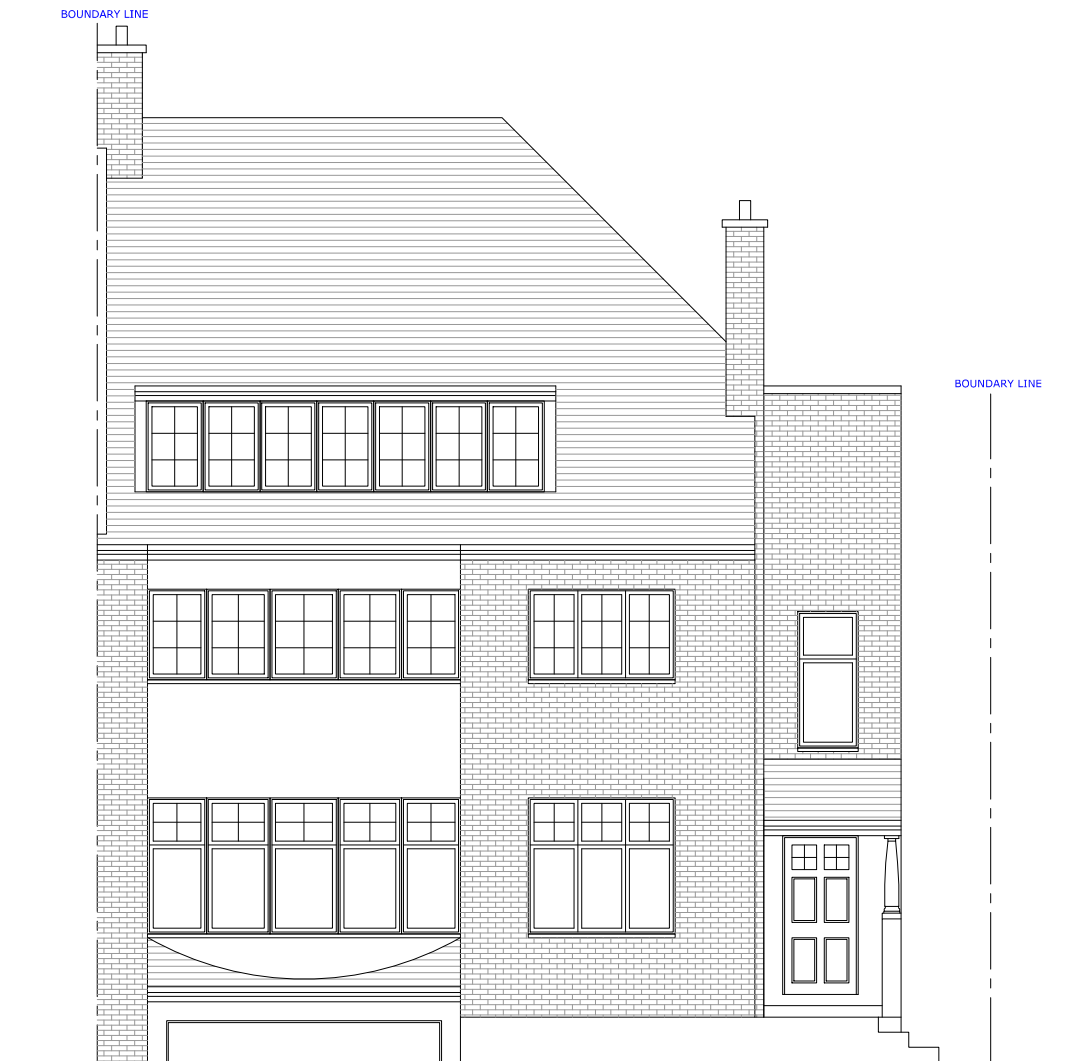
EXISTING FRONT ELEVATION SCALE 1:100
