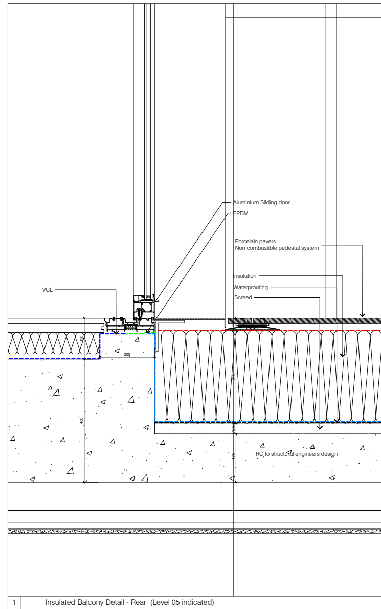
1 Insulated Balcony Detail - Rear (Level 05 indicated)
