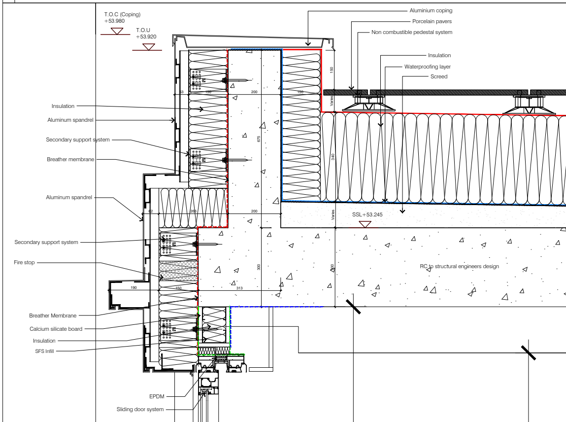
3 Parapet Detail - Level 09 North Elevation
