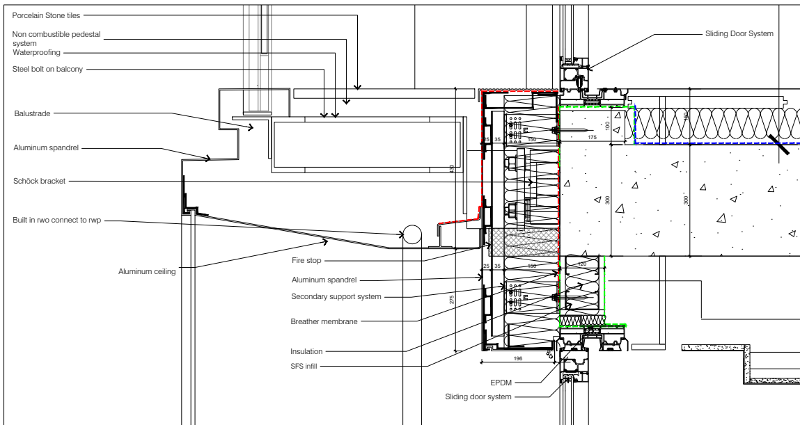
2 Projecting balcony detail - Level 08 North Elevation
