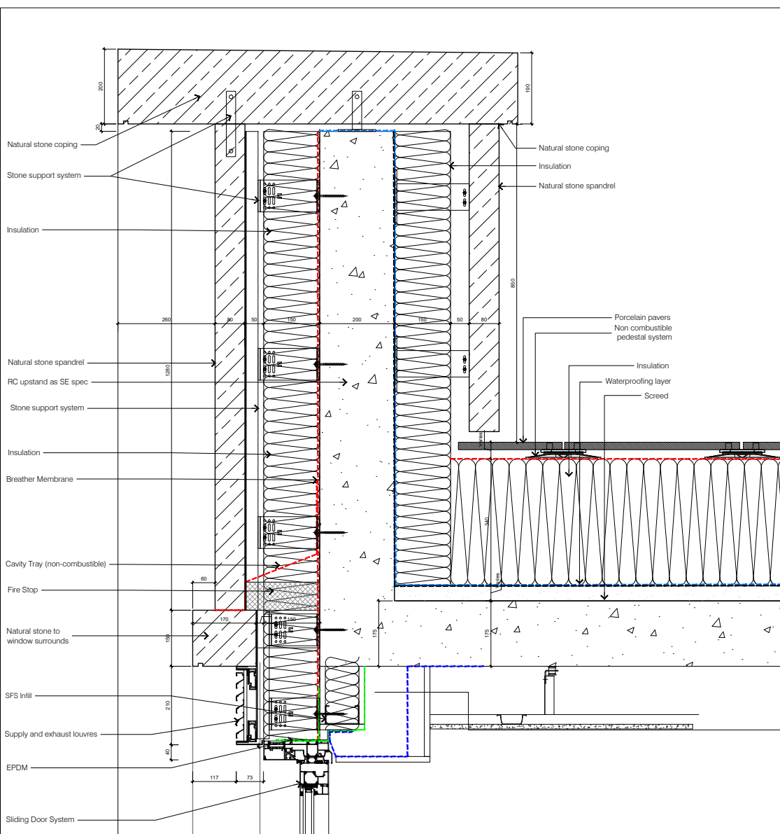
3 External Detail - Portland Stone Spandrel Panel - Level 06 North Elevation
