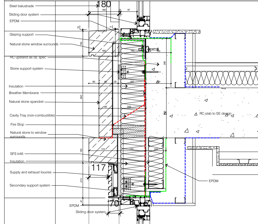
4 External Detail - Portland Stone Spandrel Panel - Level 05 North Elevation
