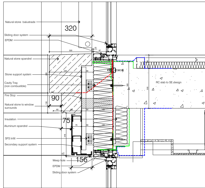
2 External Detail - Portland Stone Spandrel Panel level 02 North Elevation
