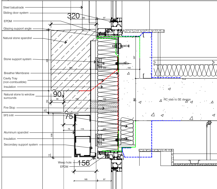
3 External Detail - Portland Stone Spandrel Panel - Level 03 North Elevation
