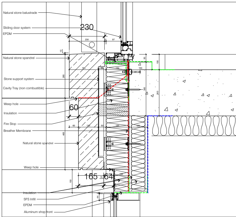
1 External Detail - Portland Stone Spandrel Panel - Level 01 North Elevation
