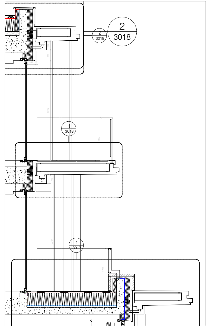
2 BAY STUDY - Detail Section level 7 to roof
