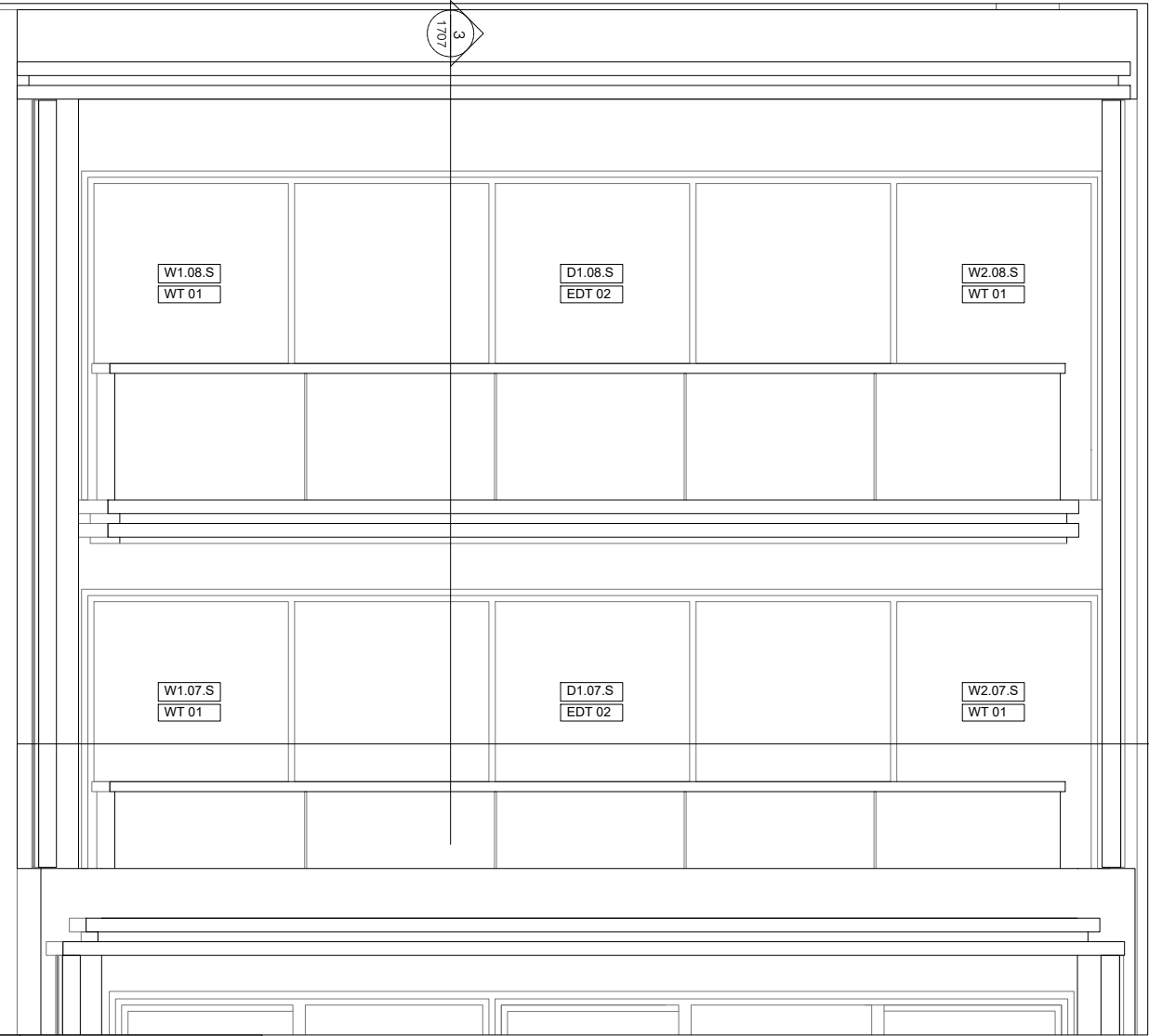
1 BAY STUDY - South Detail Elevation
