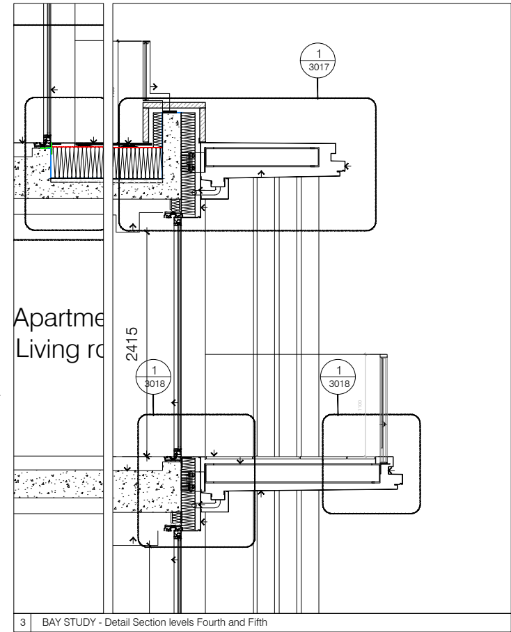
3 BAY STUDY - Detail Section levels Fourth and Fifth
