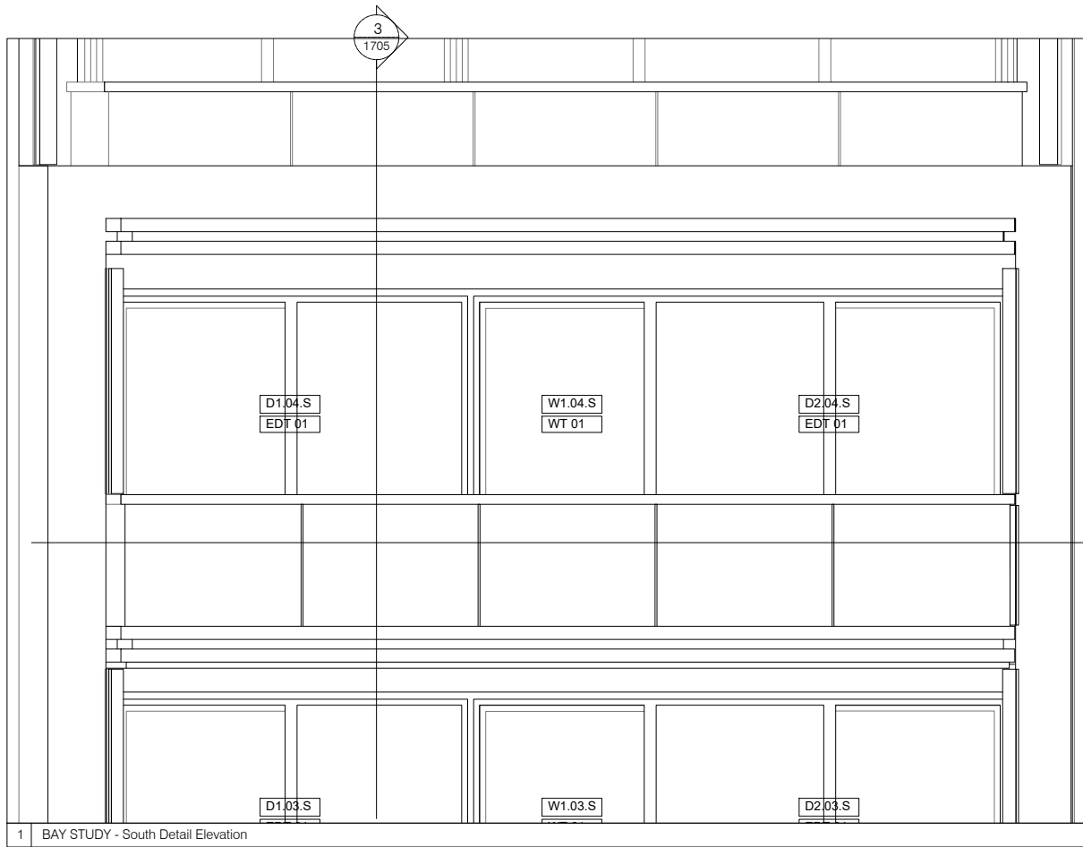
1 BAY STUDY - South Detail Elevation
