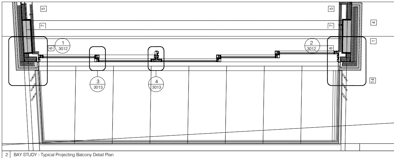
2 BAY STUDY - Typical Projecting Balcony Detail Plan
