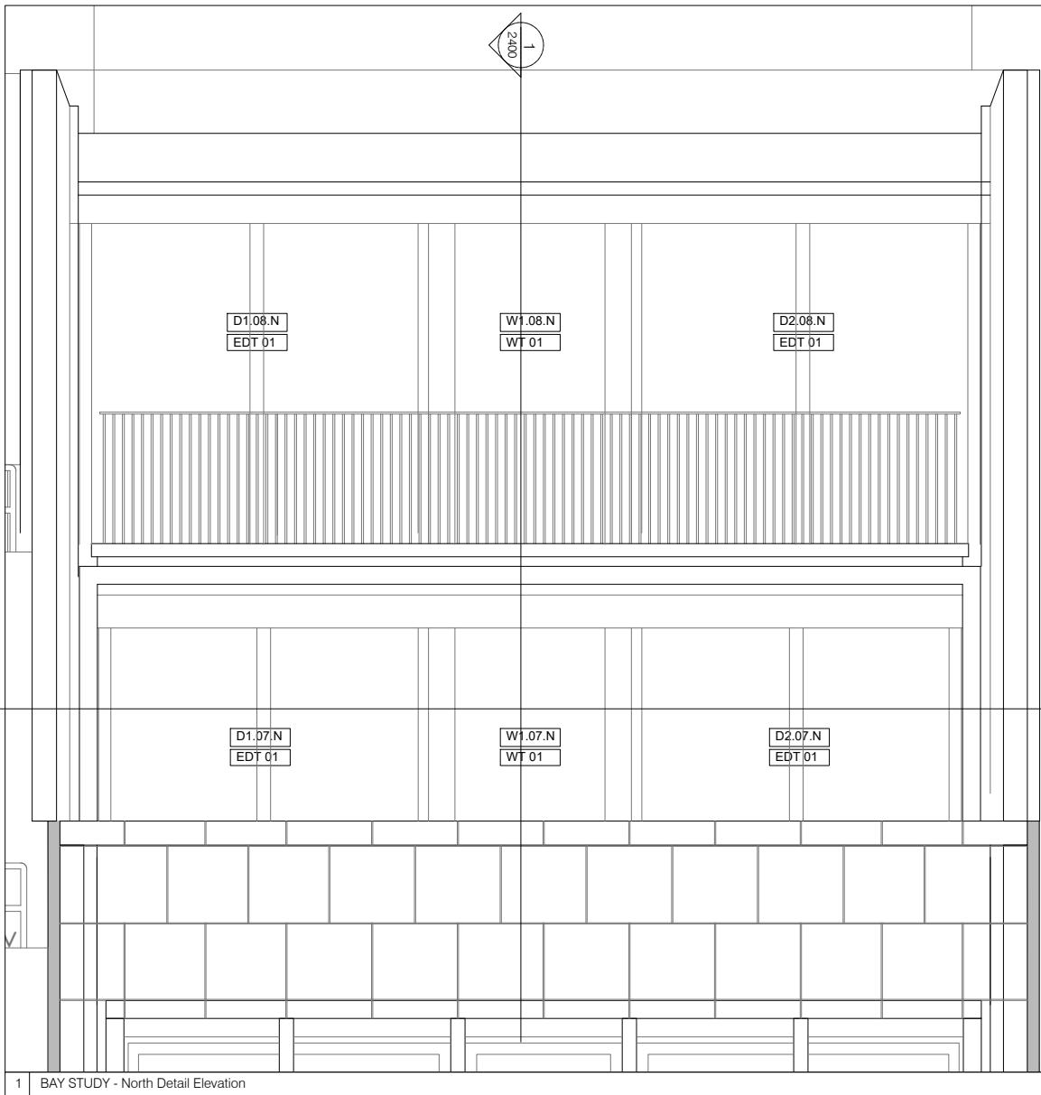
1 BAY STUDY - North Detail Elevation
