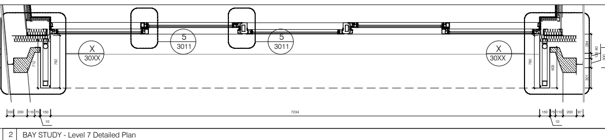
2 BAY STUDY - Level 7 Detailed Plan
