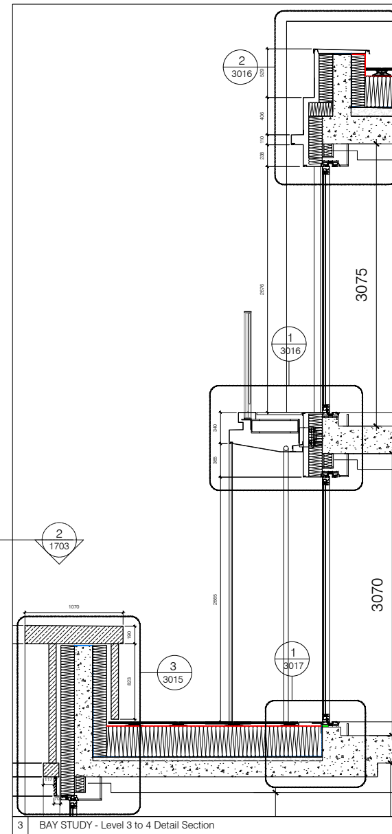
3 BAY STUDY - Level 3 to 4 Detail Section
