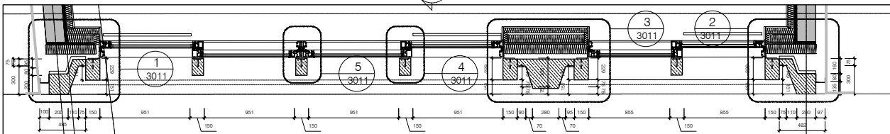
2 BAY STUDY - First Detail Plan
