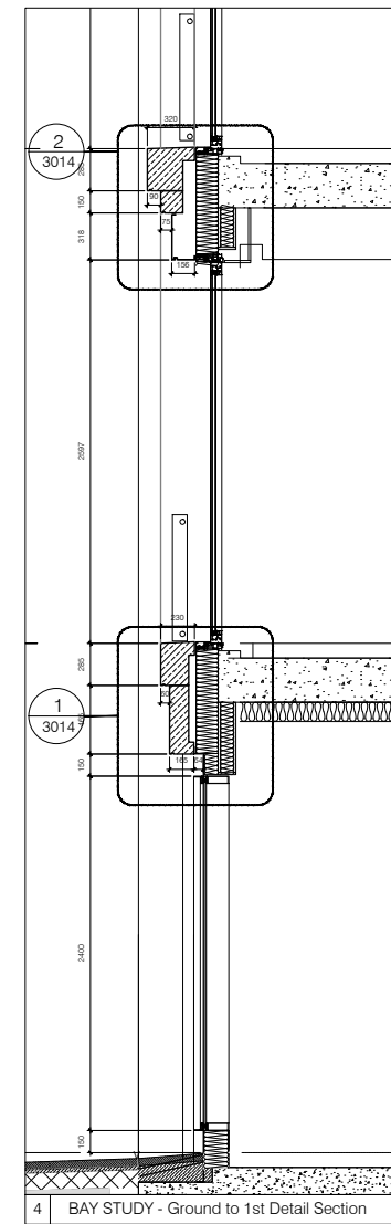
4 BAY STUDY - Ground to 1st Detail Section
