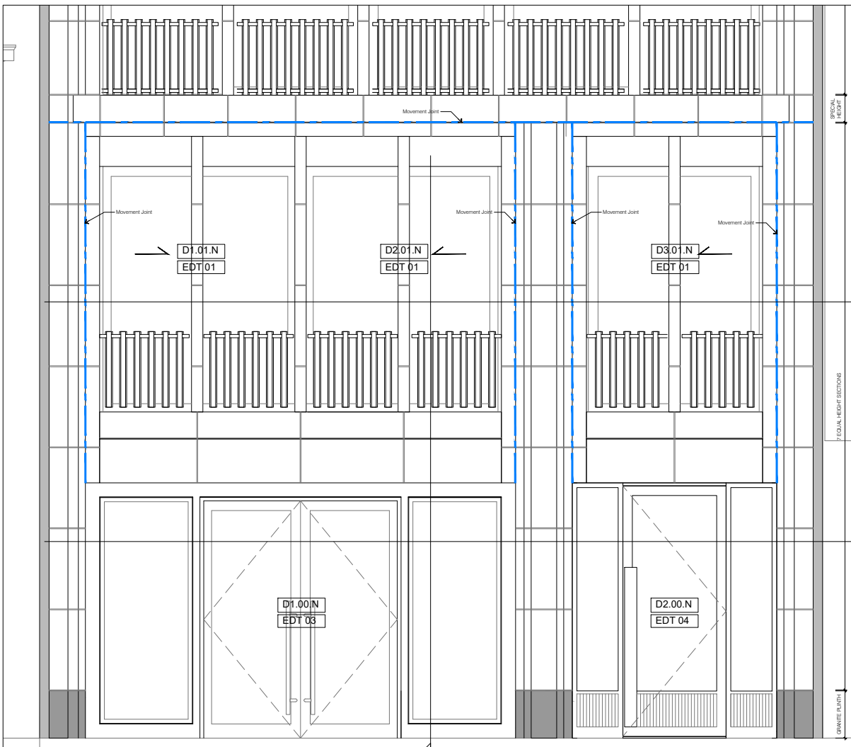
1 BAY STUDY - North Detail Elevation
