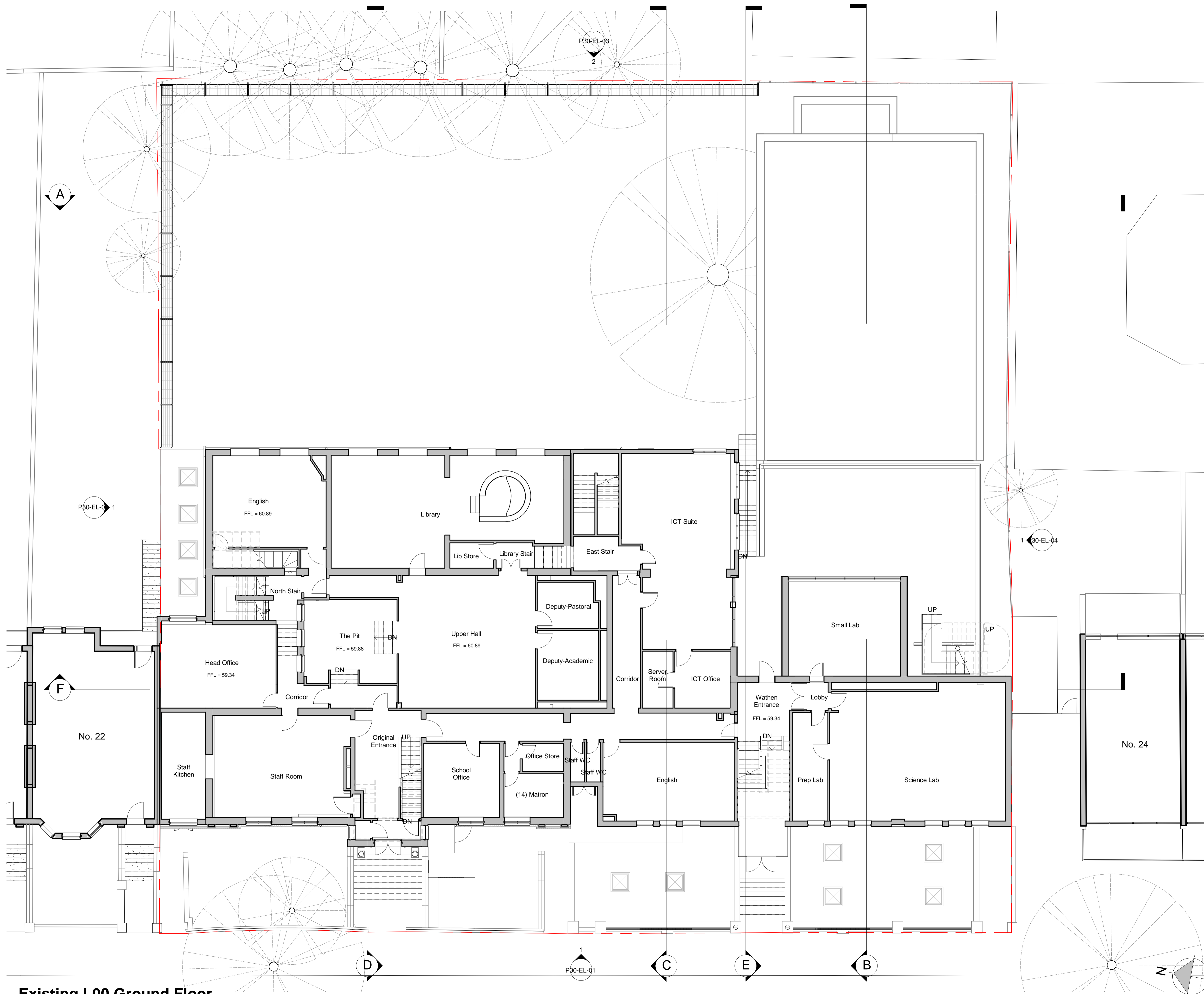
Existing L00 Ground Floor 1 : 100
