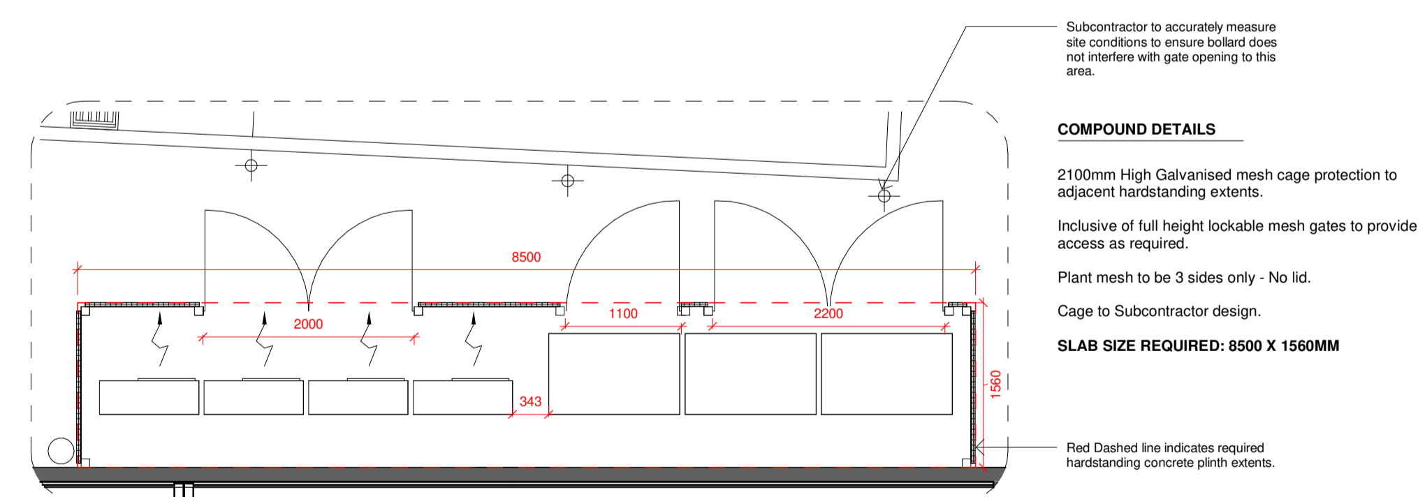
3 Plant Compound - Mechanical 1:50
