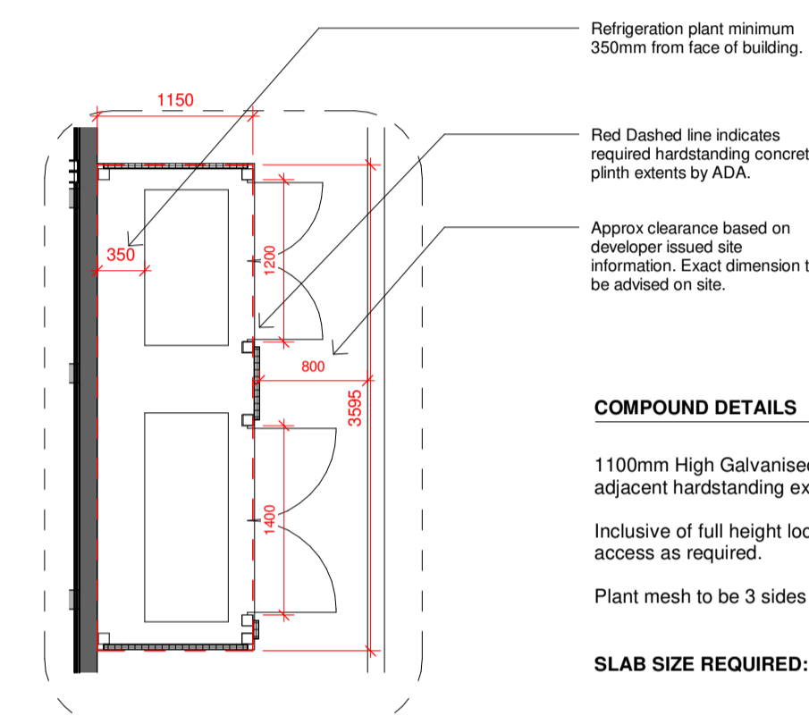
2 Plant Compound - Refrigeration 1:50
