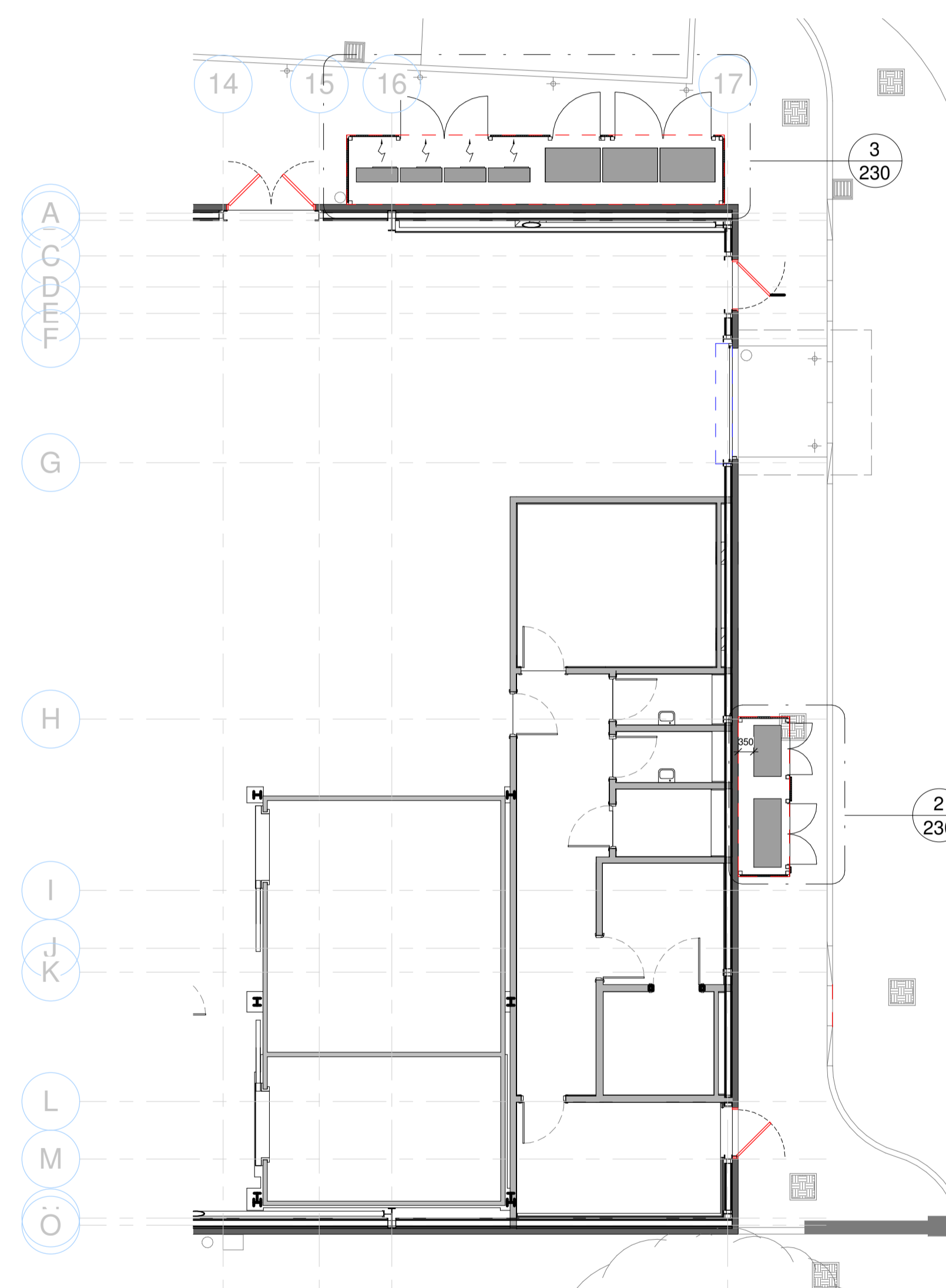
1 Plant Compound Plan 1:100
