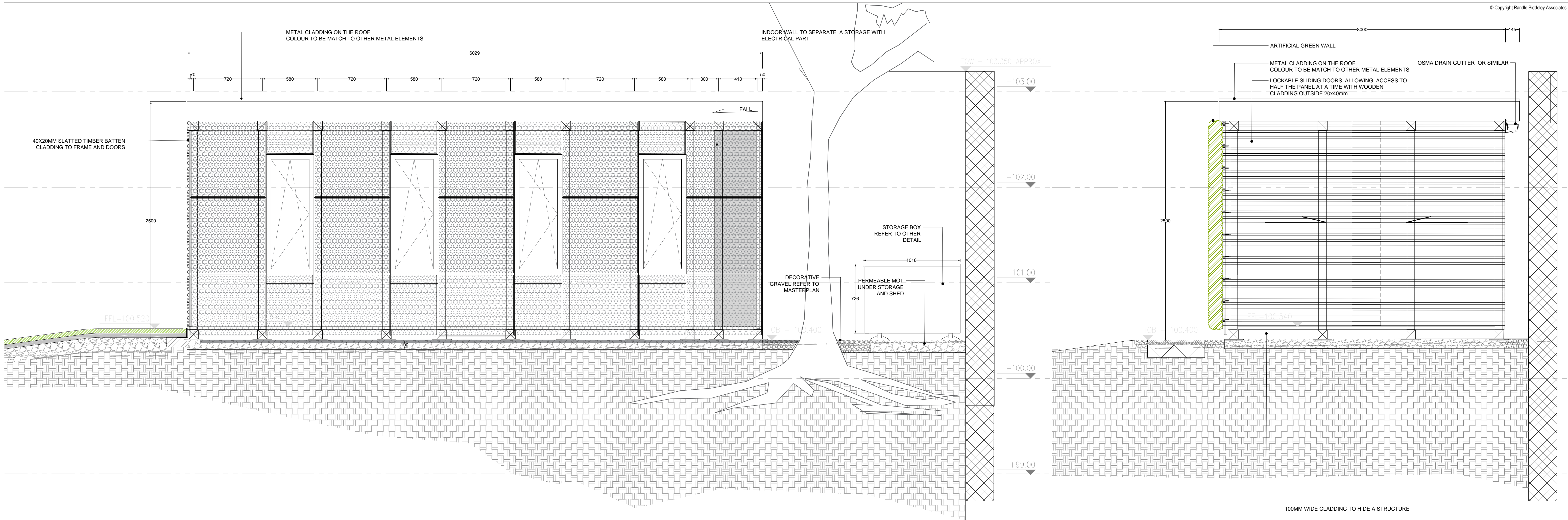
01 SOUTH SHED ELEVATION
