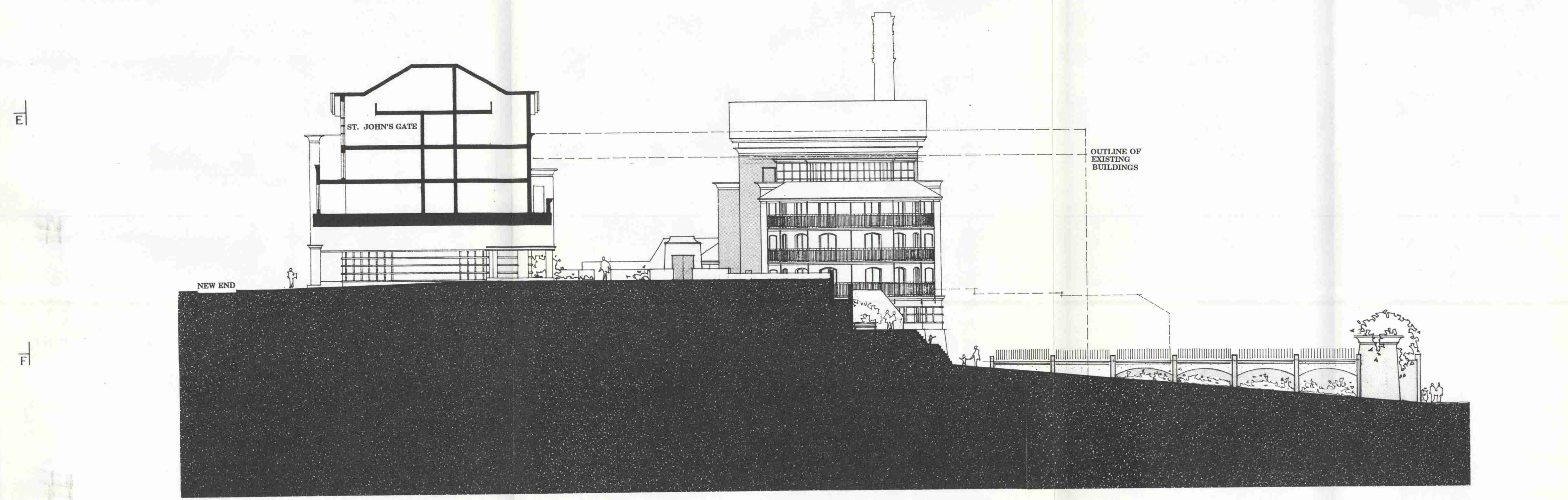
SECTION HH
