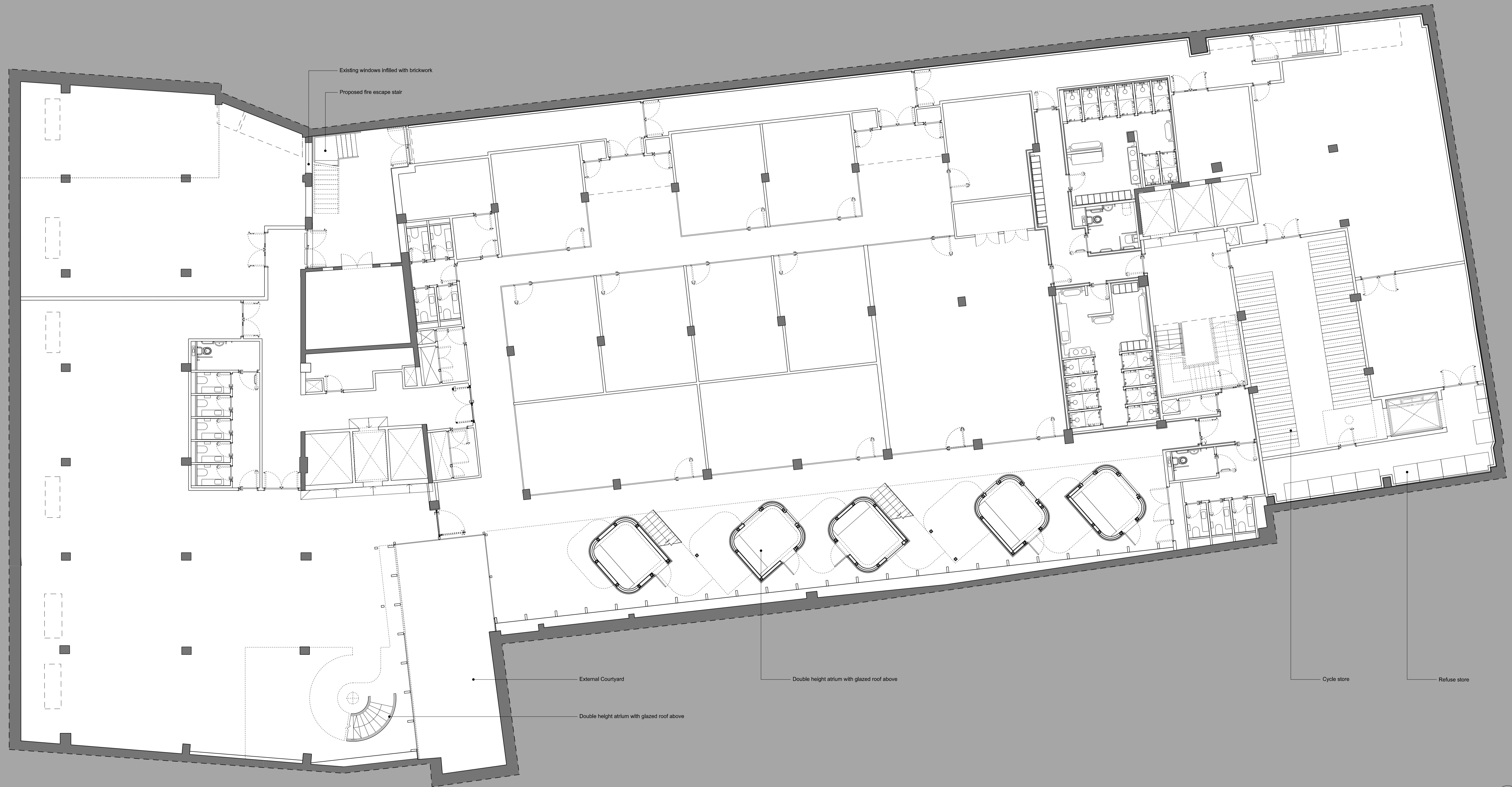
01 Basement Floor GA Plan 1:100
