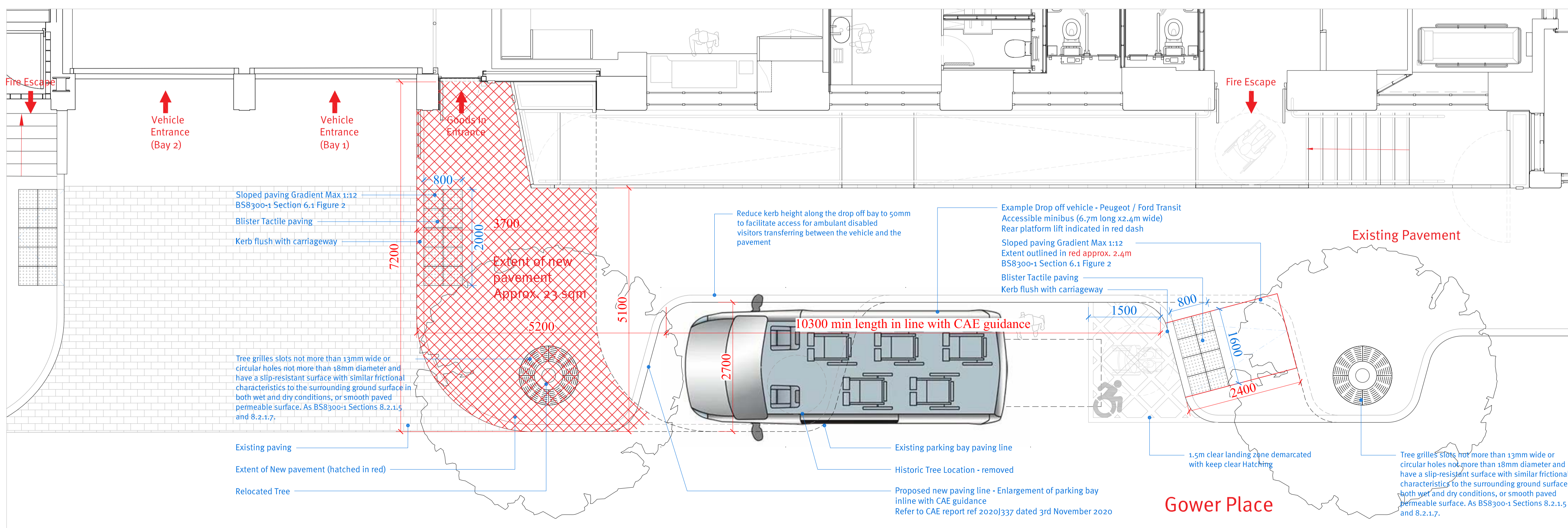
02 Proposed Detail Plan 1:50 @ A1
