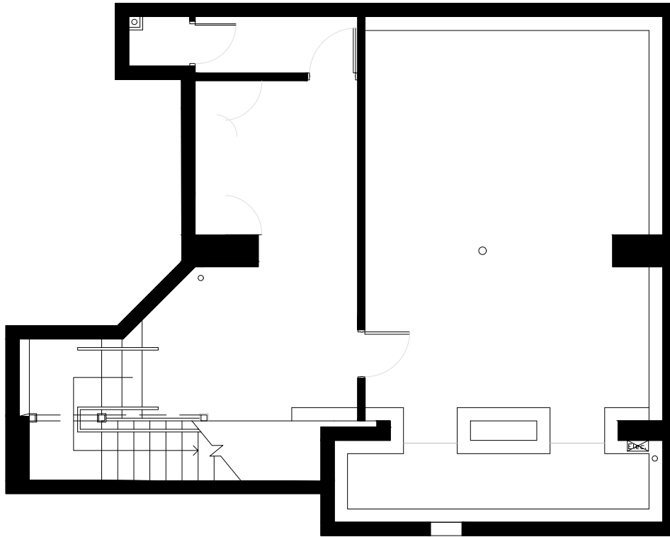
1 Proposed Ground Floor Plan 1:100 @ A4
