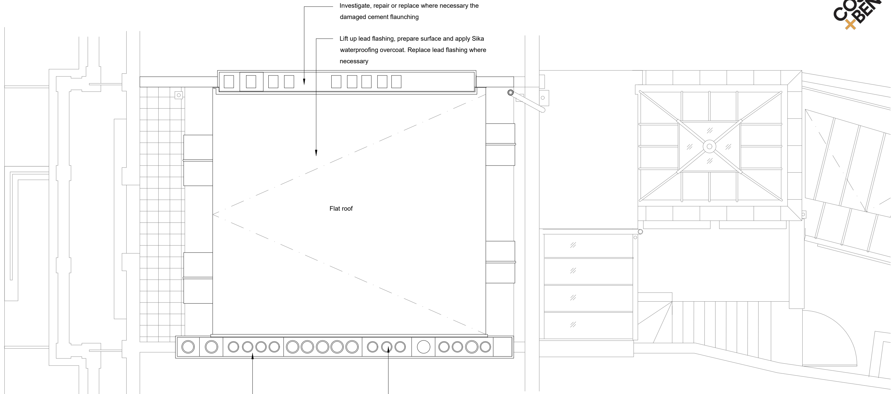
01 20.206 Proposed Roof Plan Scale 1:50 @ A3
