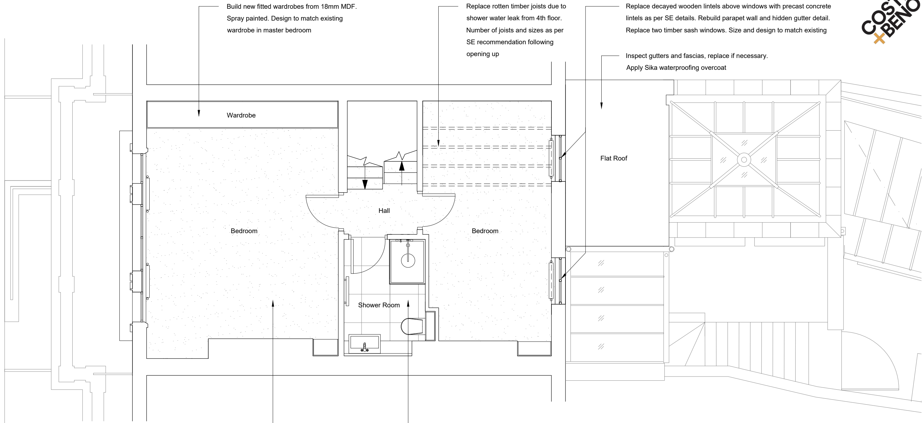
01 20.204 Proposed Third Floor Plan Scale 1:50 @ A3
