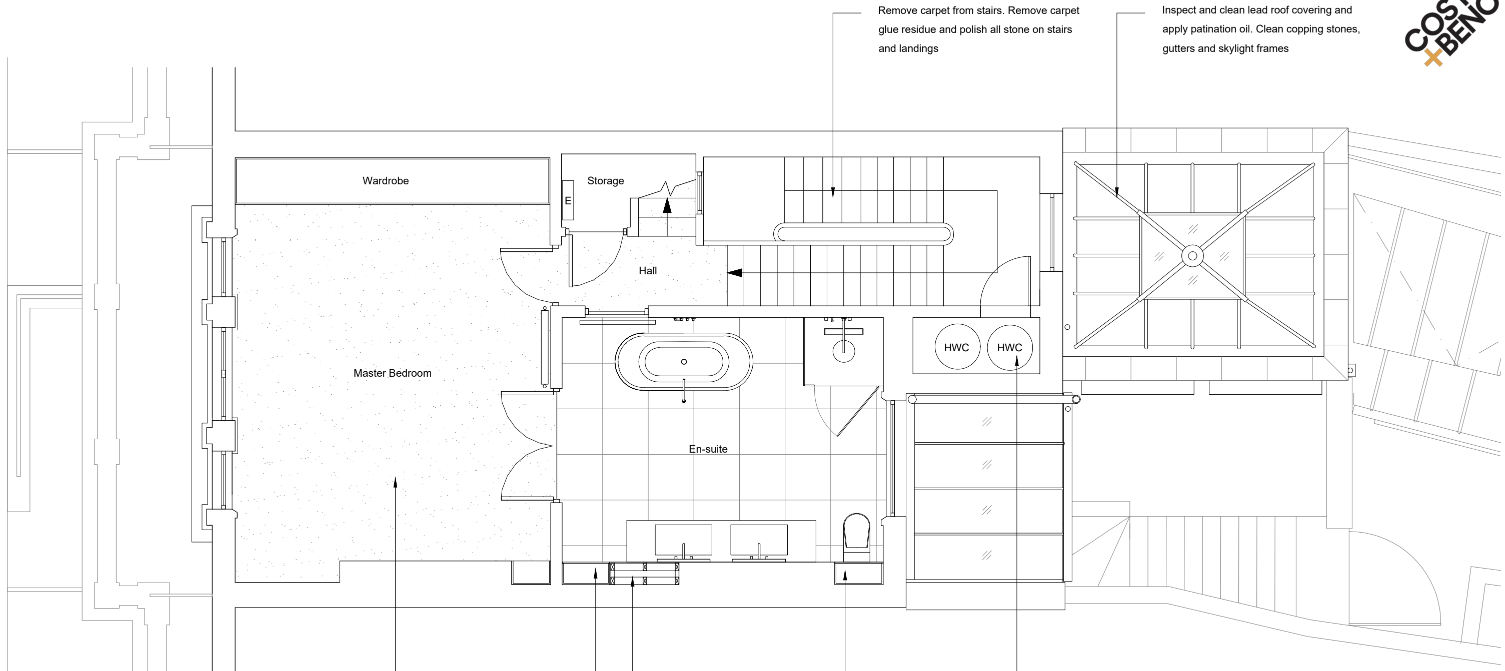
01 20.203 Proposed Second Floor Plan Scale 1:50 @ A3
