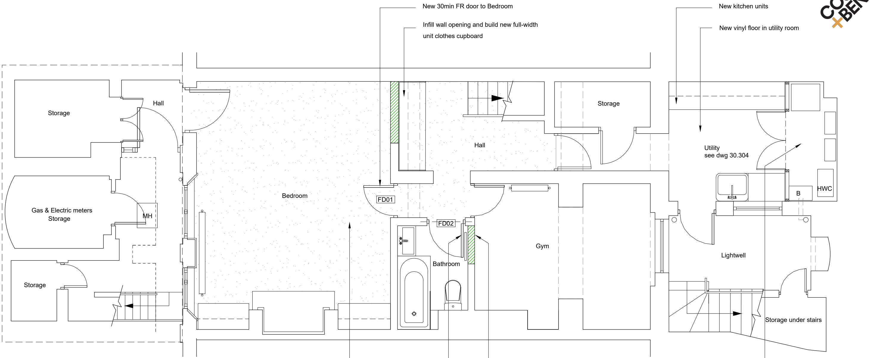
01 Proposed Lower Ground Floor Plan 20.200 Scale 1:50 @ A3
