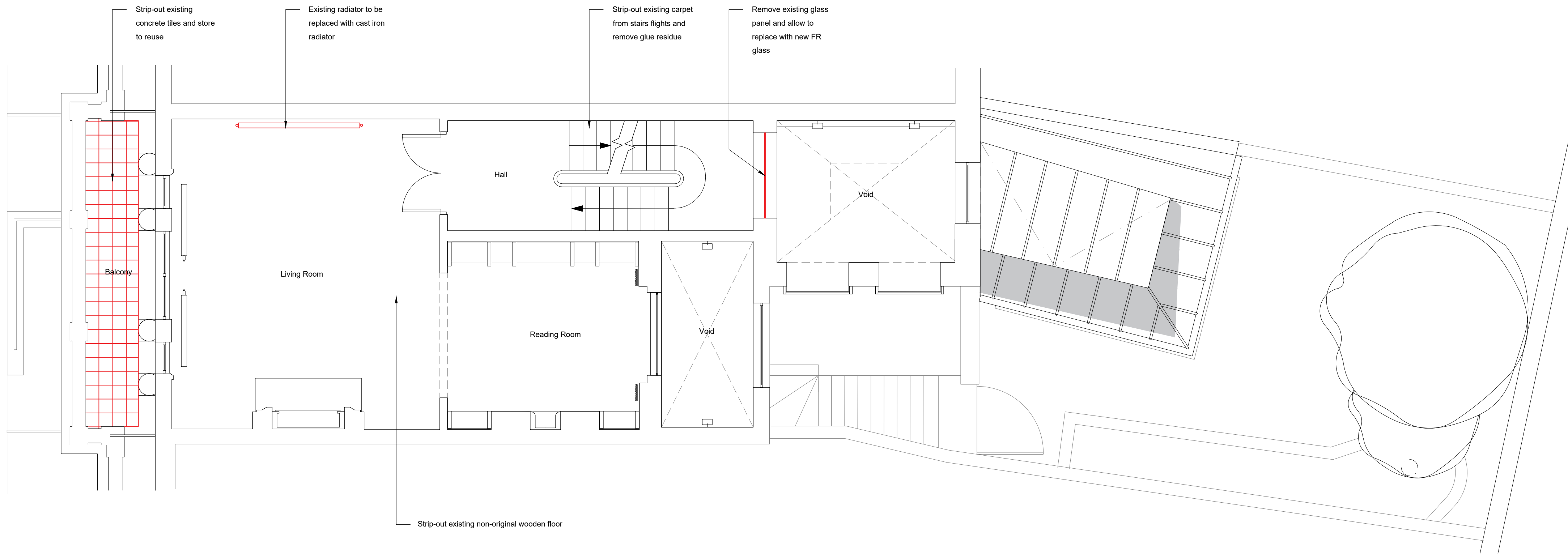
01 Existing First Floor Plan 10.202 Scale 1:50 @ A2
