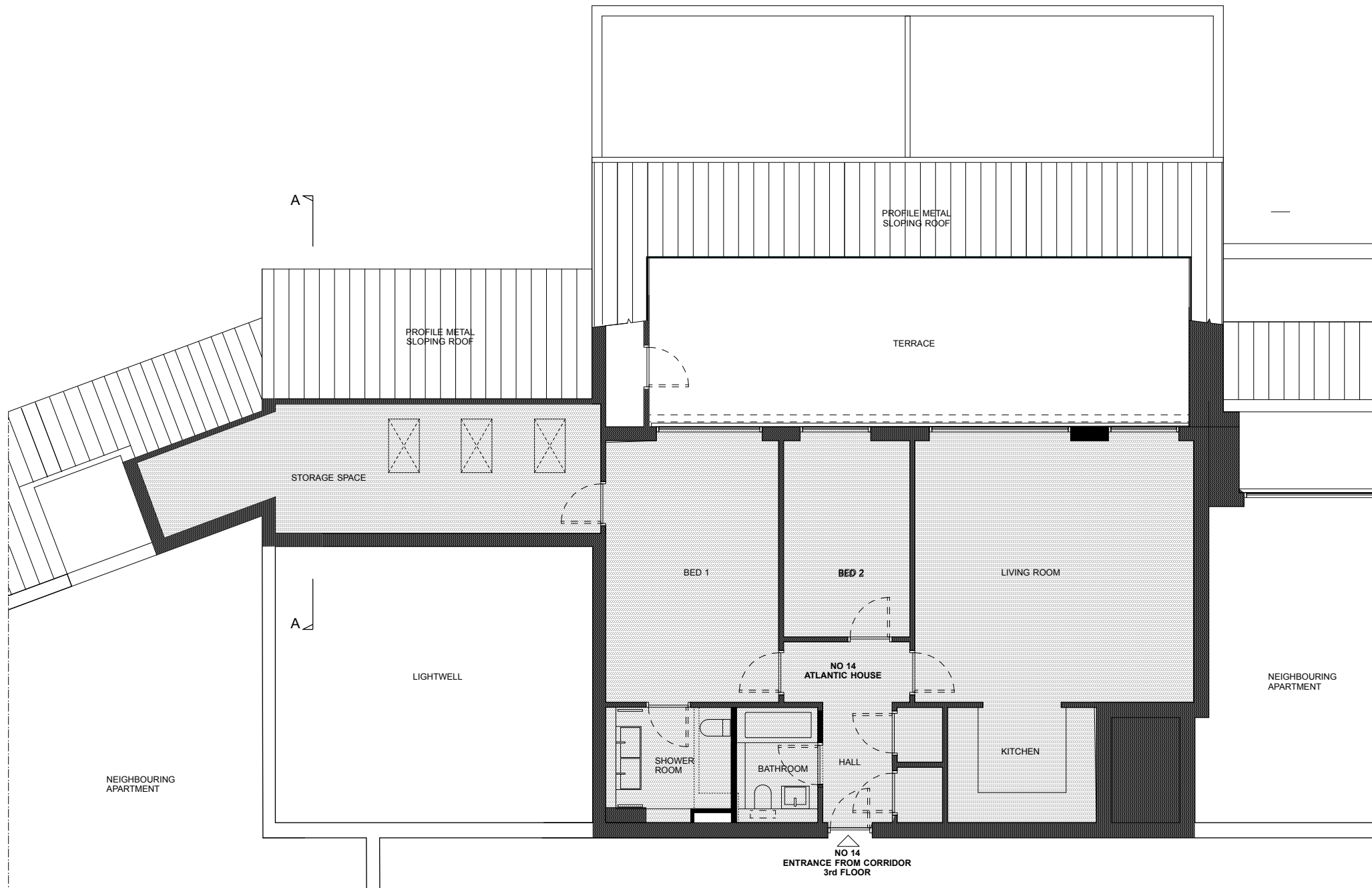
FLAT 14 - ATLANTIC HOUSE - THIRD FLOOR PLAN: EXISTING
