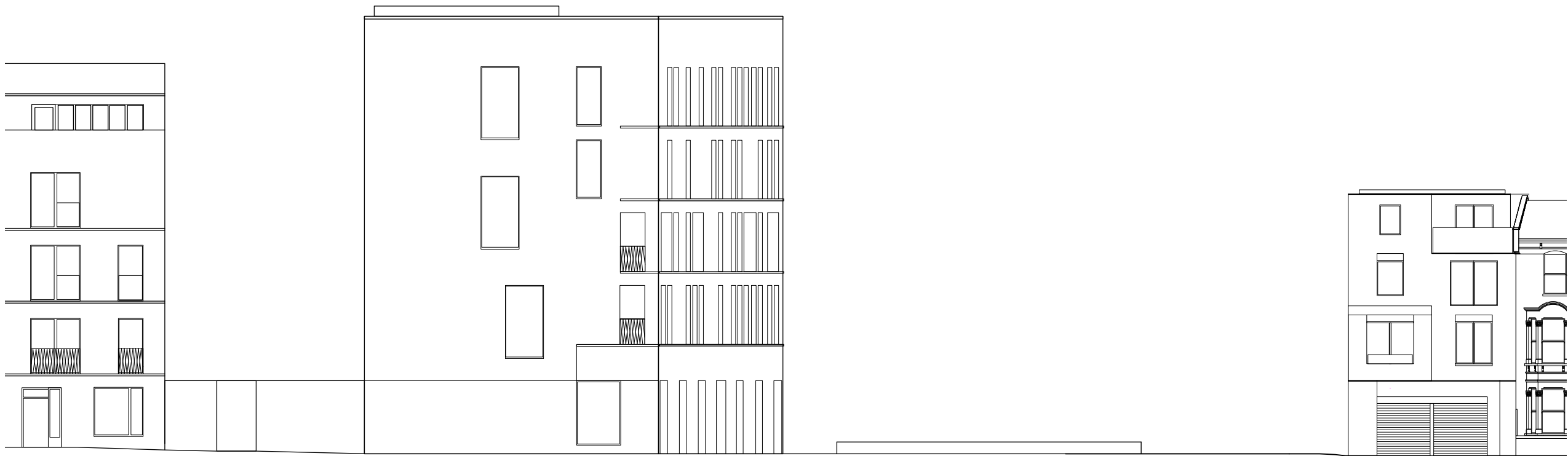
1 PROPOSED STREET ELEVATION - AGAR GROVE ESTATE 1:200@A3
