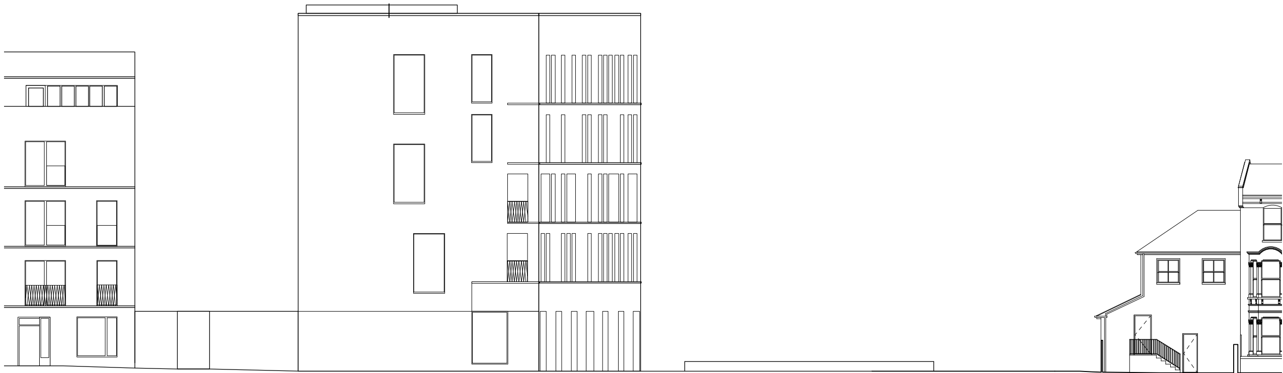
1 EXISTING STREET ELEVATION - AGAR GROVE ESTATE 1:200@A3
