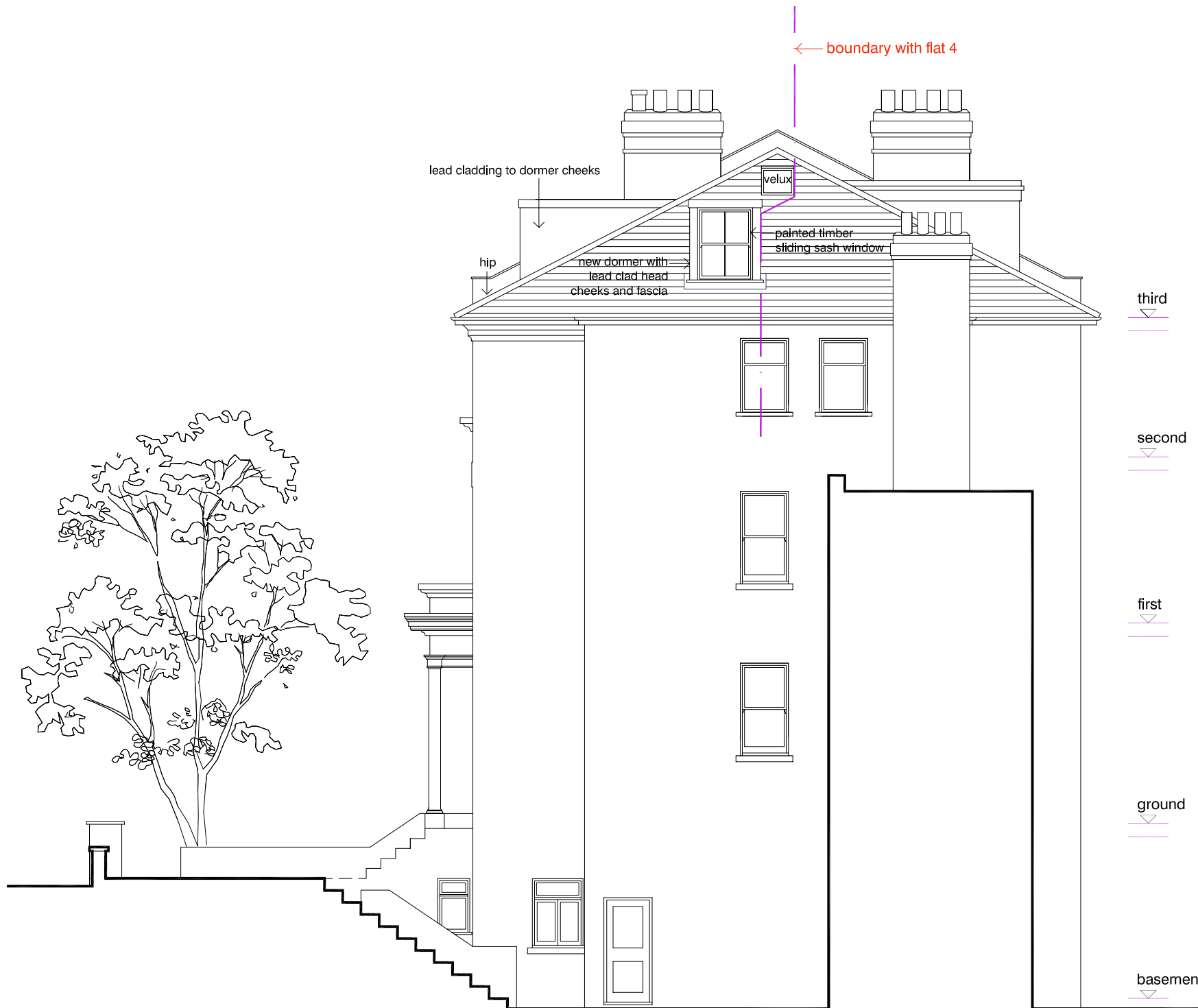
east elevation (flank)
