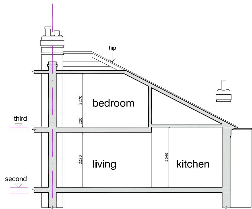
section AA existing
