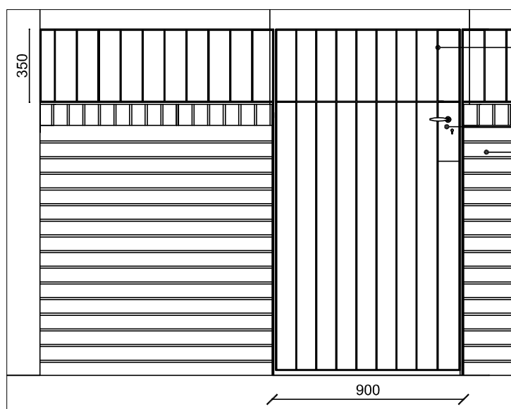
Part Front Elevation 1 to 25
