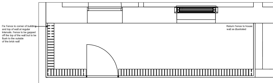
PROPOSED PLAN 1 to 50
