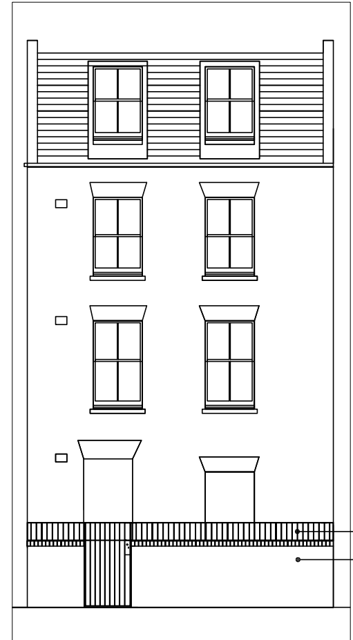
Proposed Front Elevation 1 to 100
