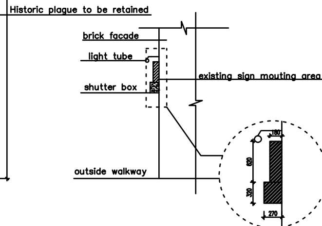
SECTION OF FRONT FACADE scale 1/100
