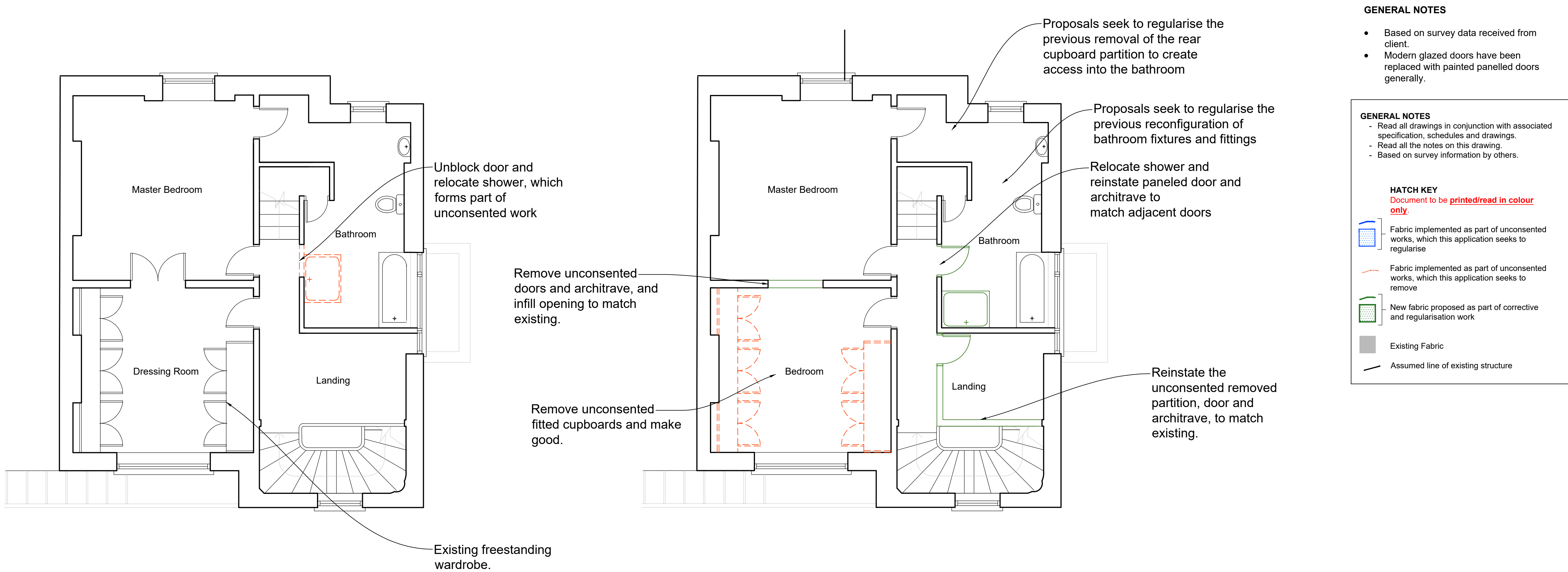
01 2001 First Floor - Existing Plan and Proposed Removal of Unconsented Work 1:50 @ A1
