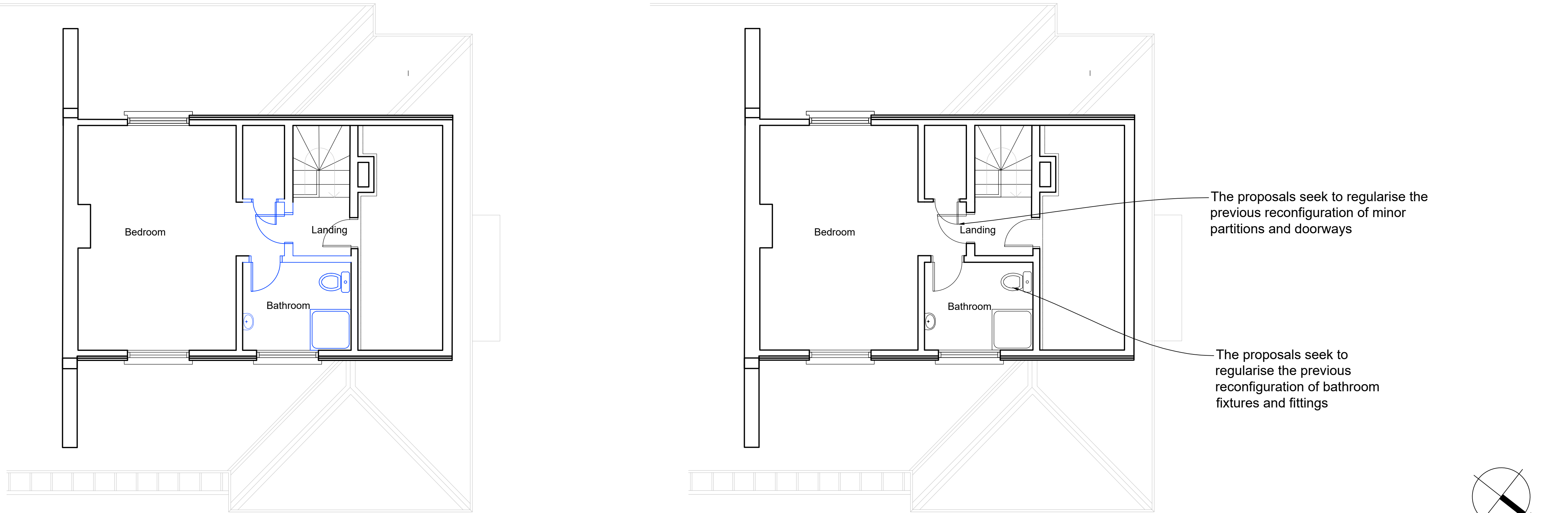
03 2001 Second Floor - Existing Plan and Proposed Removal of Unconsented Work 1:50 @ A1
