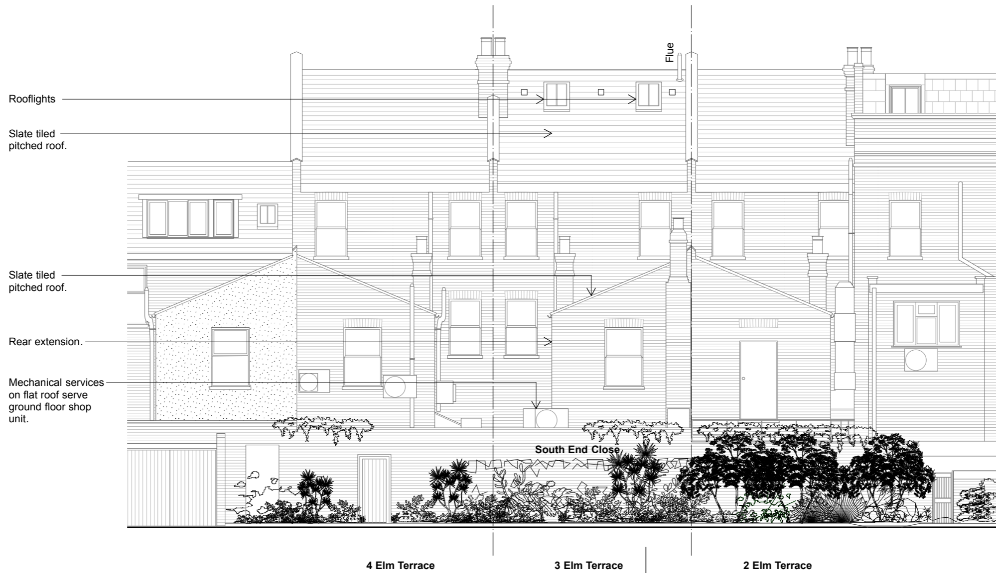
08_Rear Elevation - Existing
