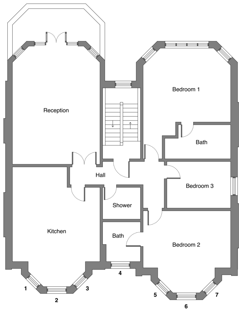
Proposed 1st Floor Plan Scale 1:100
