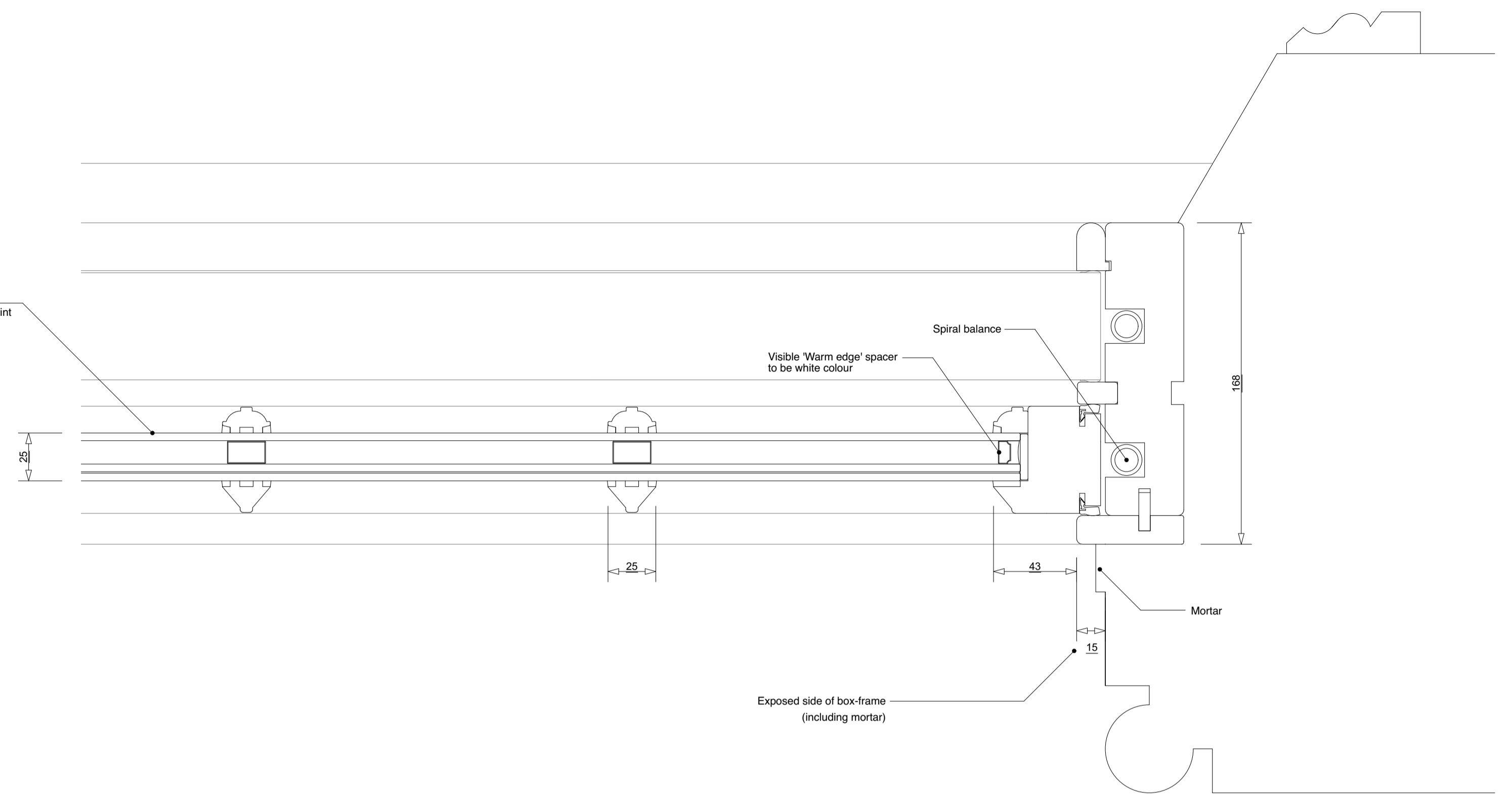
Proposed Window Jamb Scale 1:2
