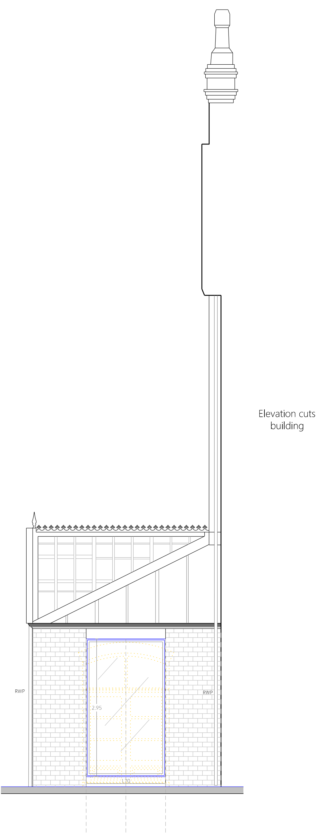
Left elevation
