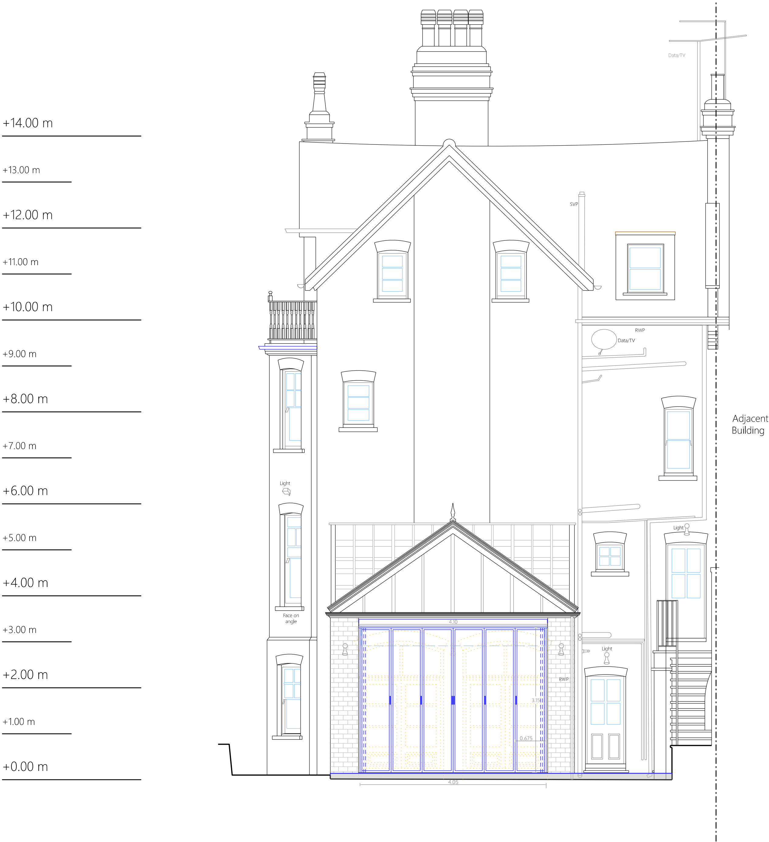
Back elevation
