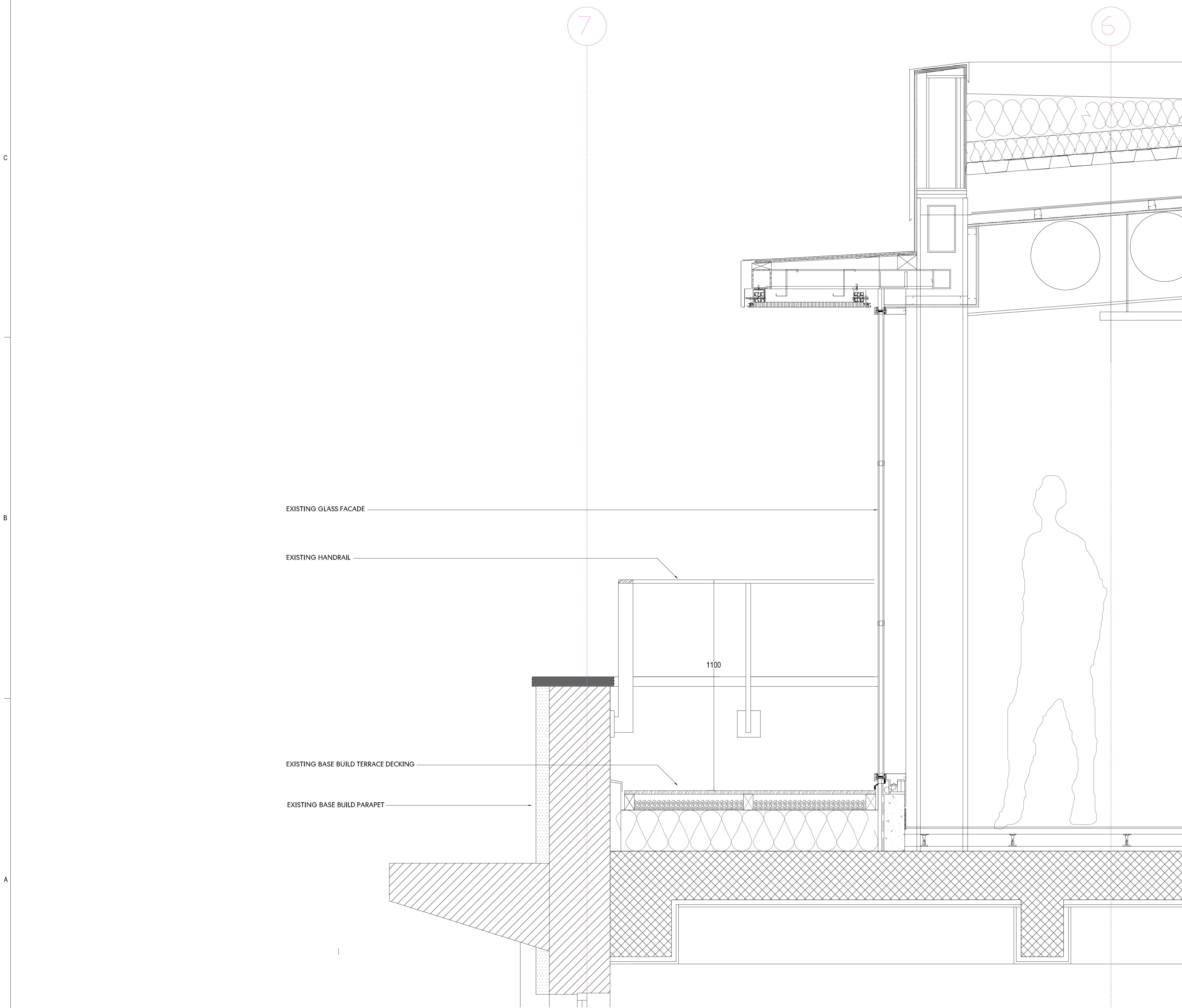
1 EXISTING DETAIL - LEVEL 06 1 : 10
