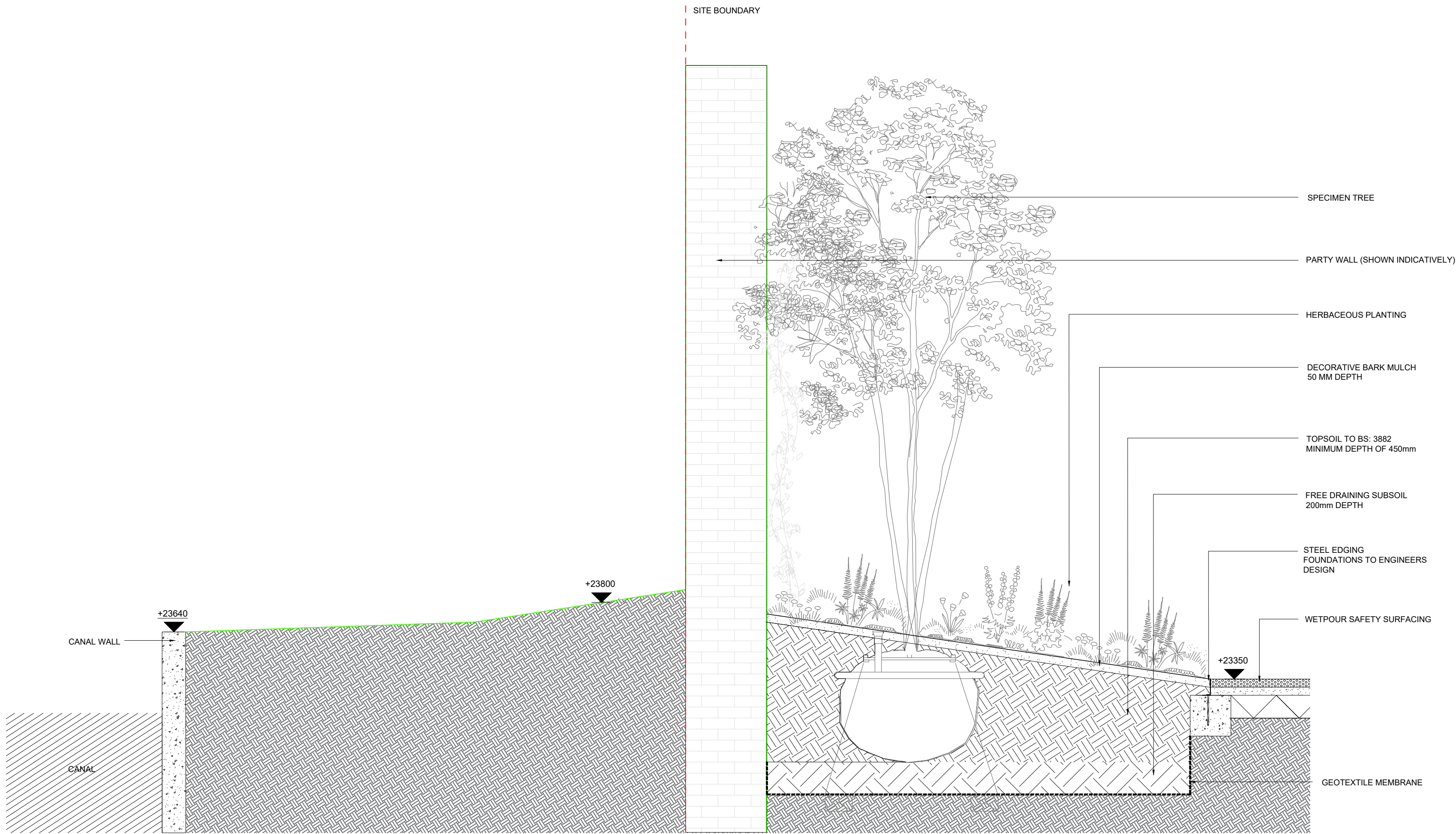
D01 230 SECTION THROUGH CANAL WALKWAY 01 SCALE 1:20
