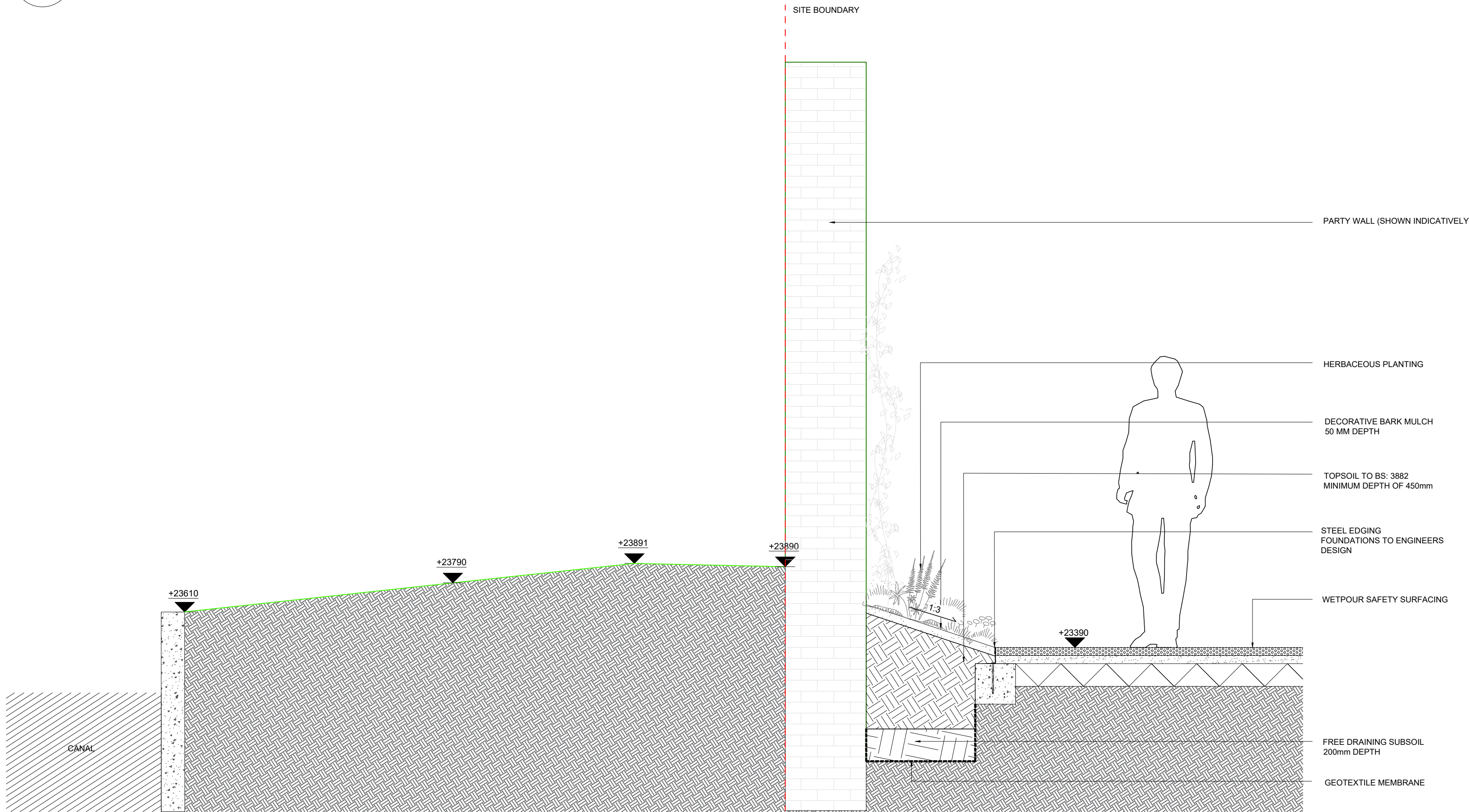
D02 230 SECTION THROUGH CANAL WALKWAY 02 SCALE 1:20
