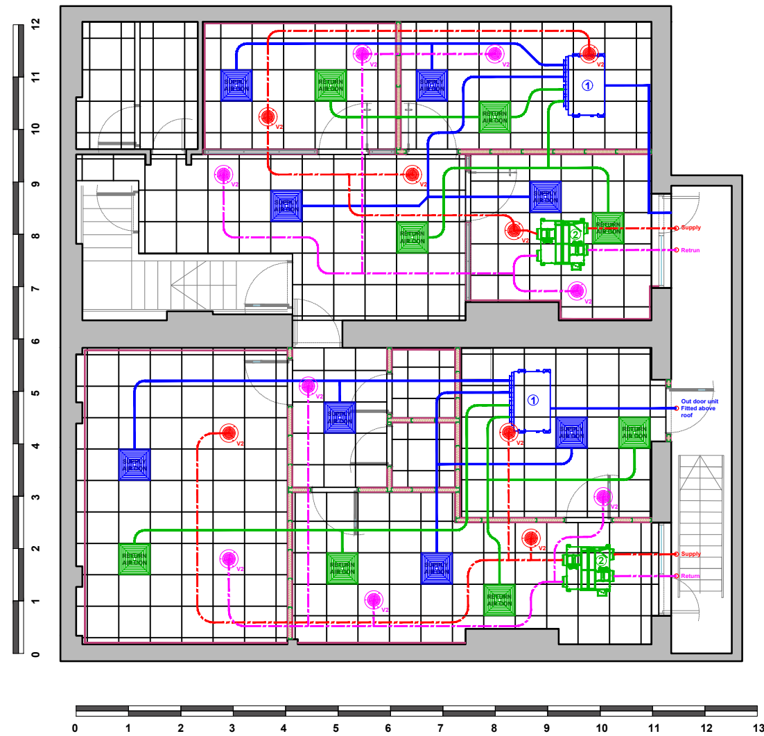
PROPOSED BASEMENT PLAN
