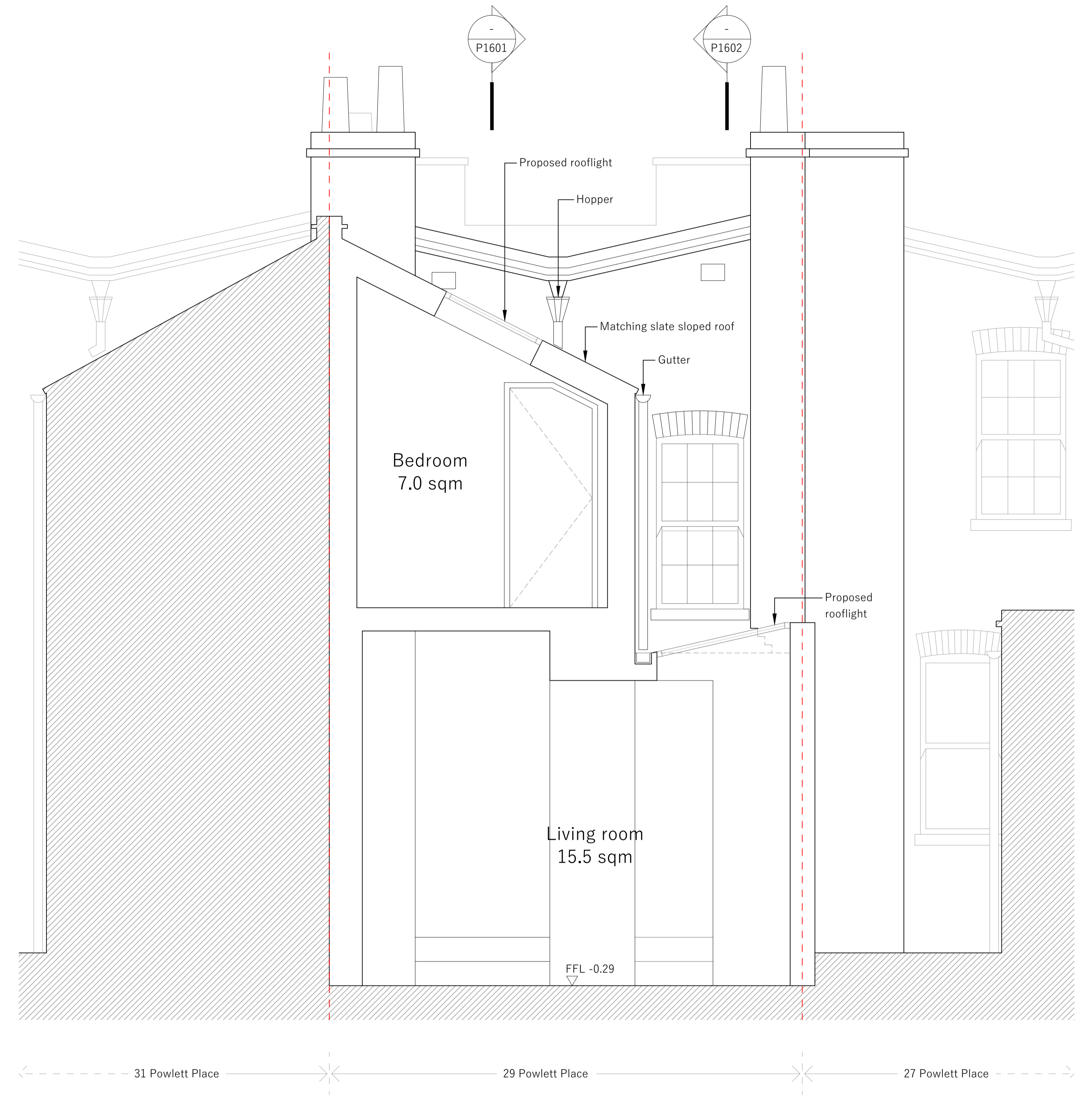
② Short section looking South
