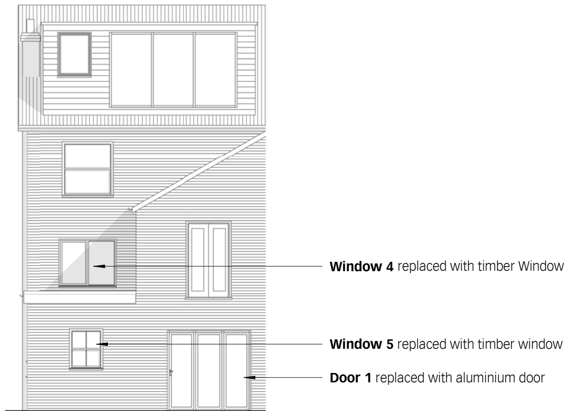
\frac{1}{PL101} Proposed Rear Elevation 1 : 100
