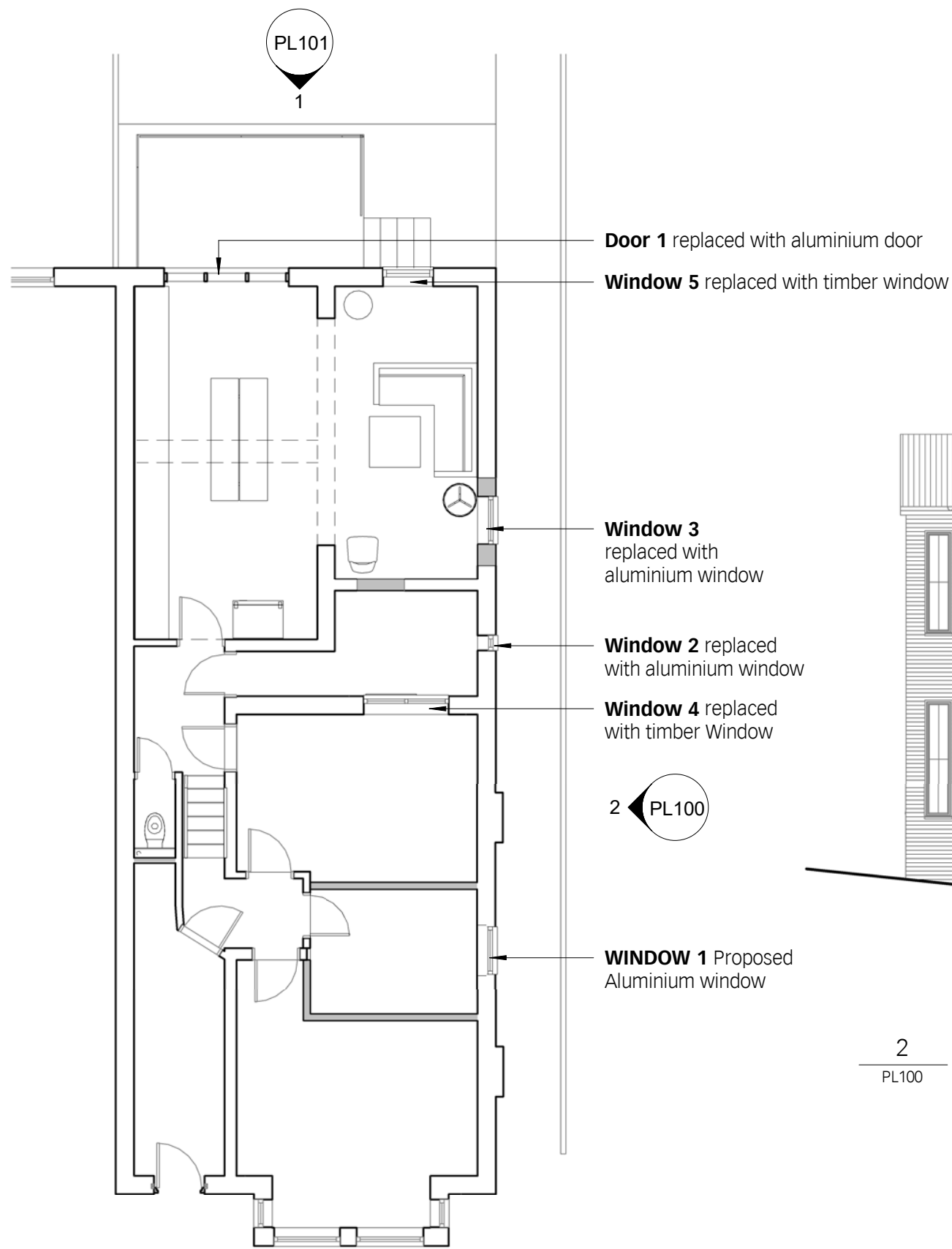
1 Proposed Ground Floor PL100 1 : 100
