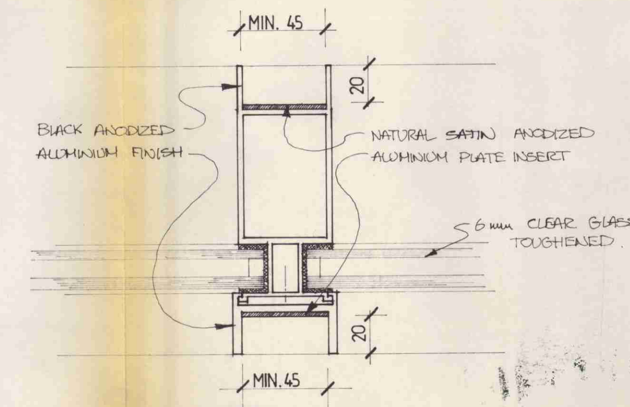
DETAIL 1 - Typical First Floor Mullion
