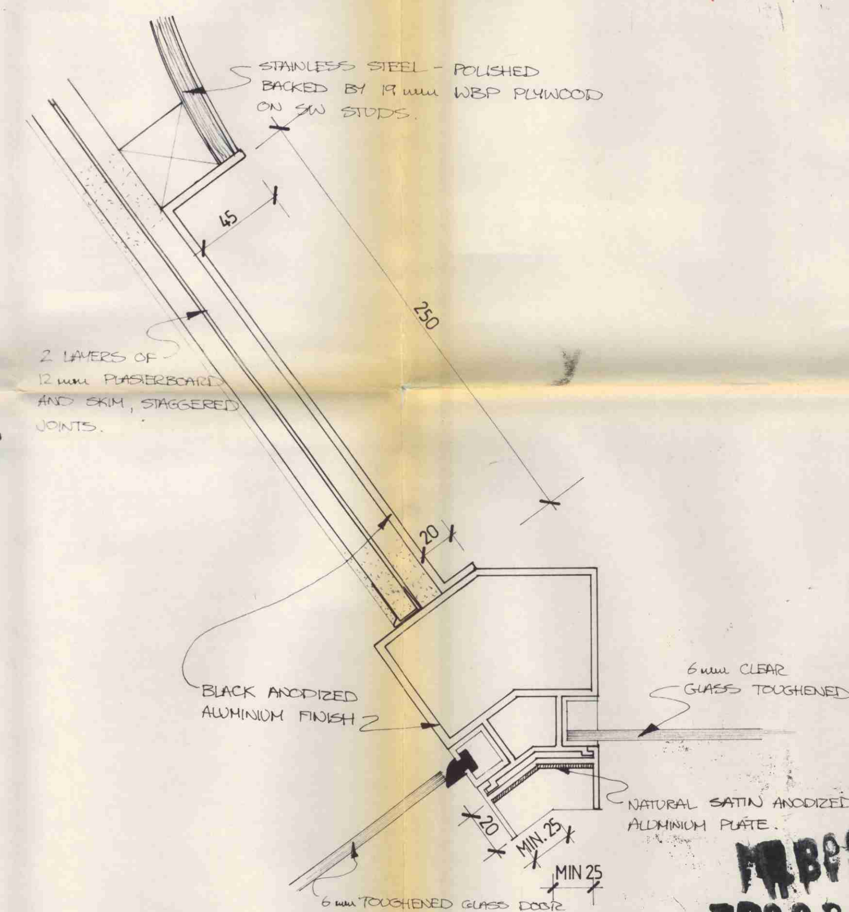
DETAIL 2 - Plan
