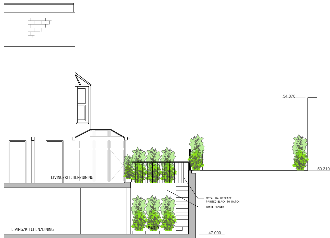
SECTION B2-B2
