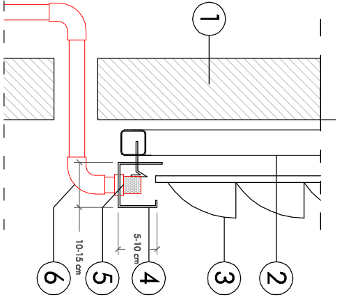
DETAIL C: GUTTER
