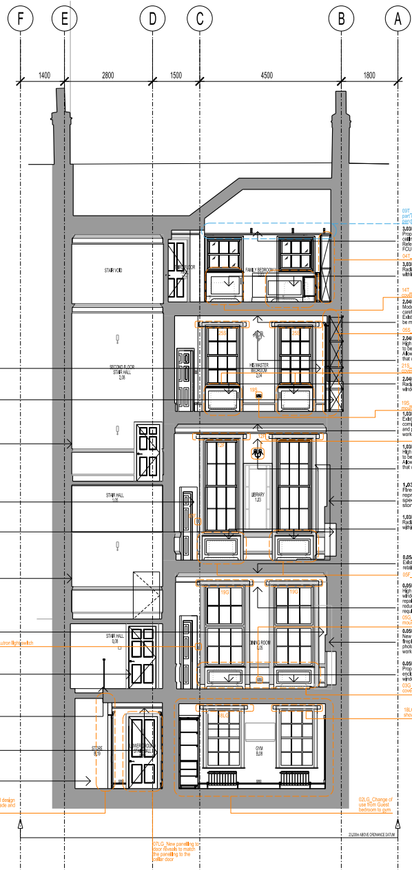
SECTION N - N
