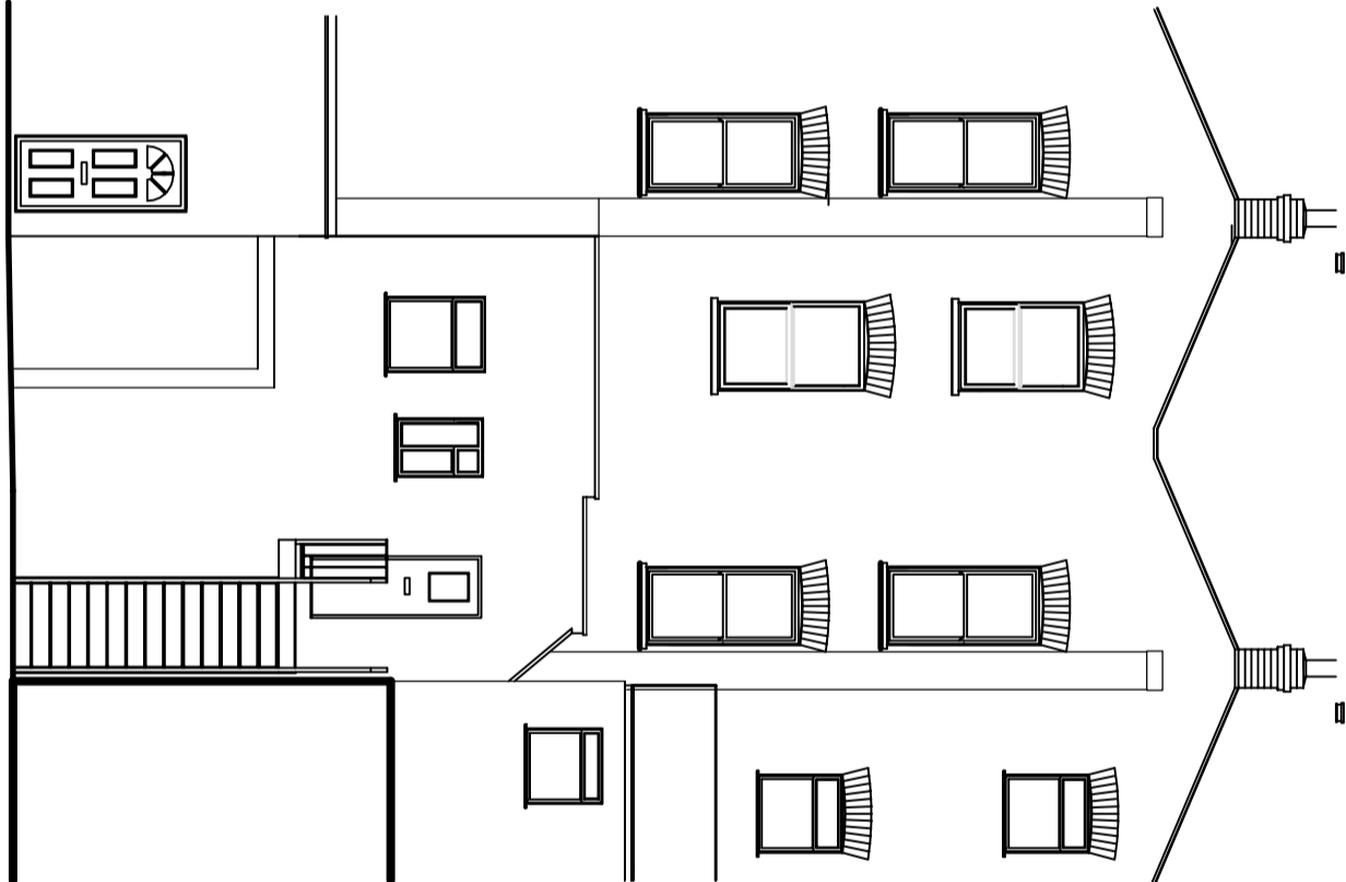
EXISTING REAR ELEVATION (FULL COURT YARD ELEVATION)
