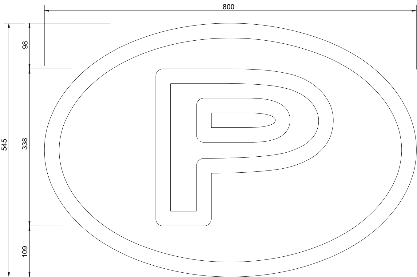
Logo sign scale 1:5@a3 EDGE ILLUMINATED SIGNAGE APPROX 300cd/m2
