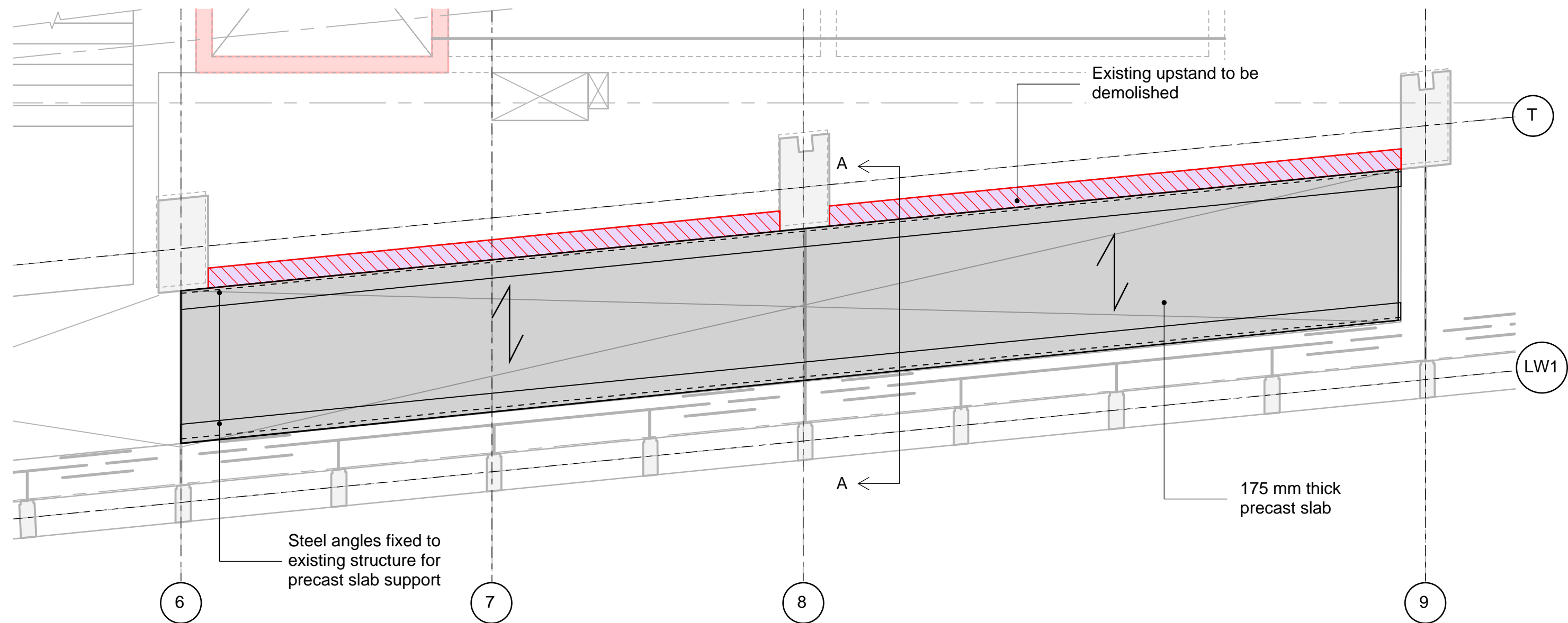
General Arrangement Plan
